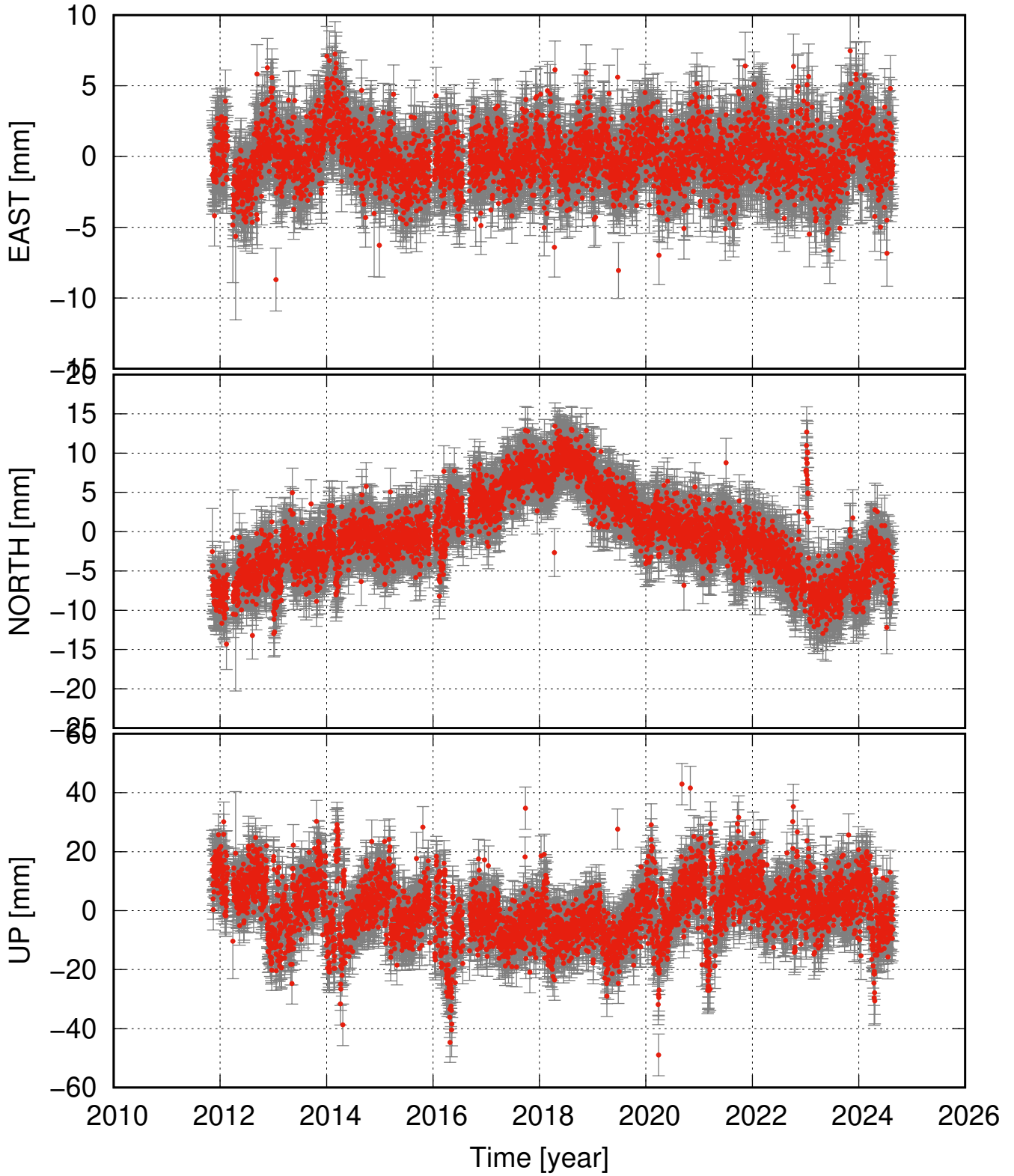
KRAC residual time series
