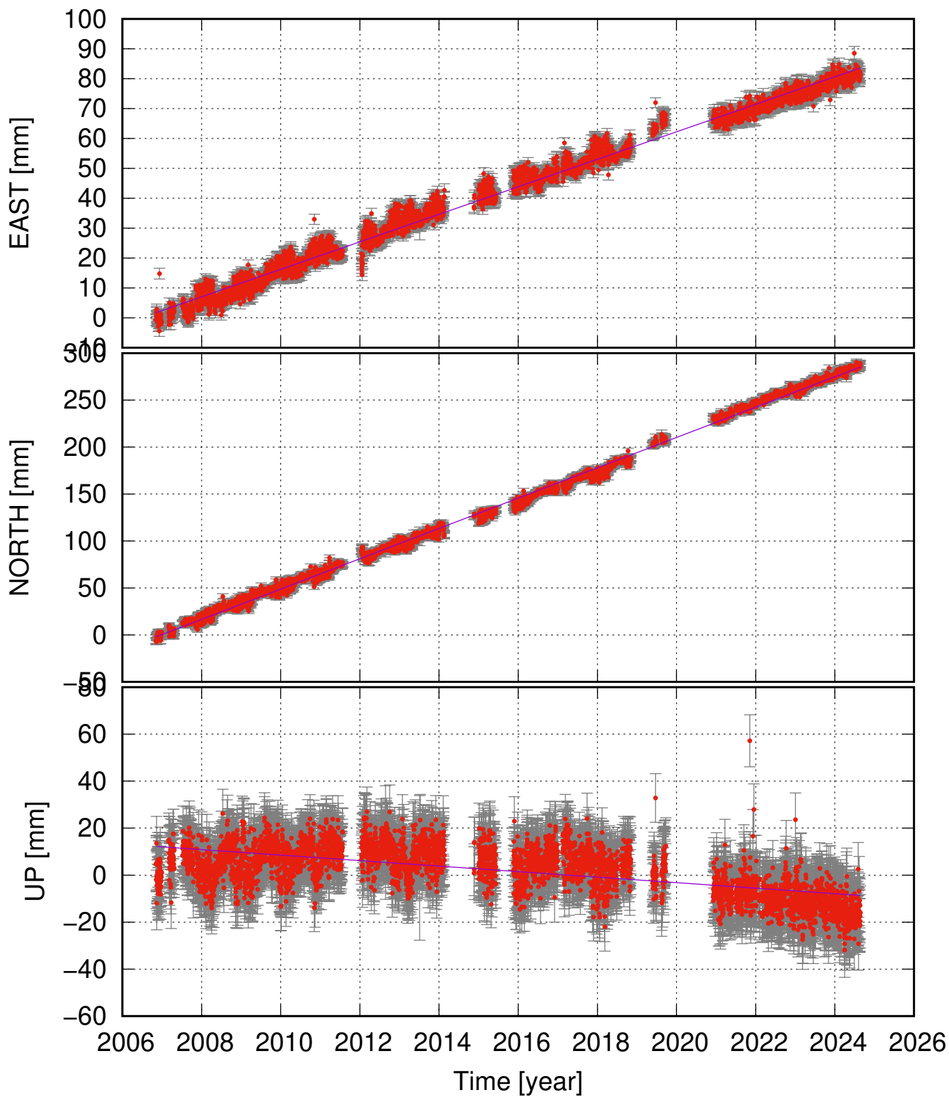
KOSK (66.30, -16.44) time series (ITRF 2014) v_e = 4.60 \pm 0.14 ; v_n = 16.14 \pm 0.24 ; v_u = -1.17 \pm 0.43 mm/yr
