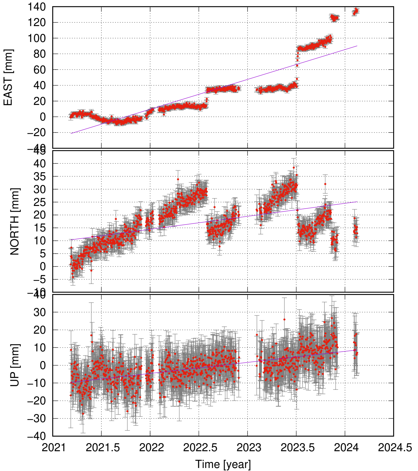
KLVC (63.91, -21.96) time series (ITRF 2014) v_e = 37.93 \pm 5.72 ; v_n = 5.03 \pm 2.38 ; v_u = 6.24 \pm 2.11 mm/yr
