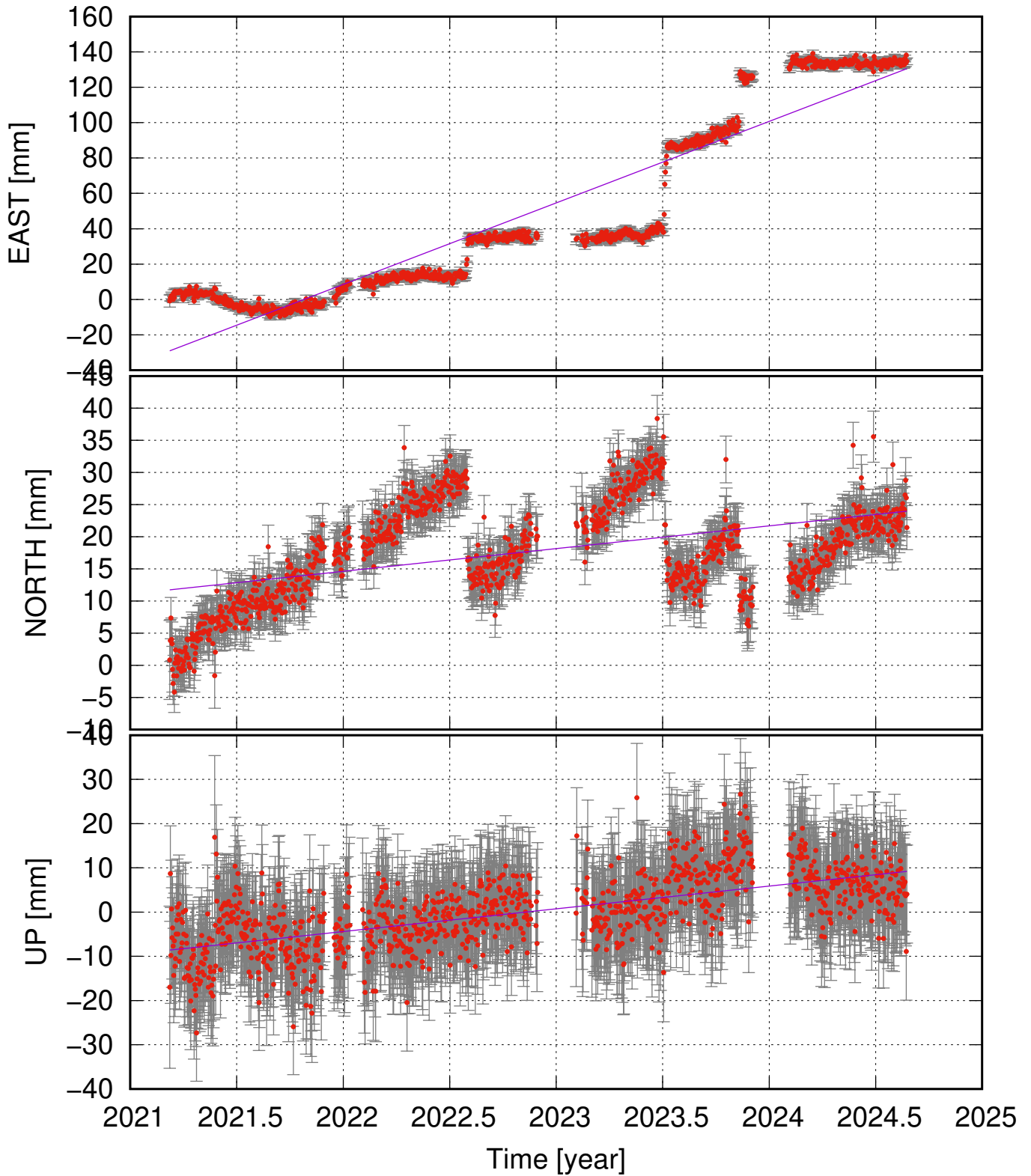
KLVC (63.91, -21.96) time series (ITRF 2014) ve = 46.12 ± 5.22; vn = 3.54 ± 1.95; vu = 5.14 ± 1.78 mm/yr
