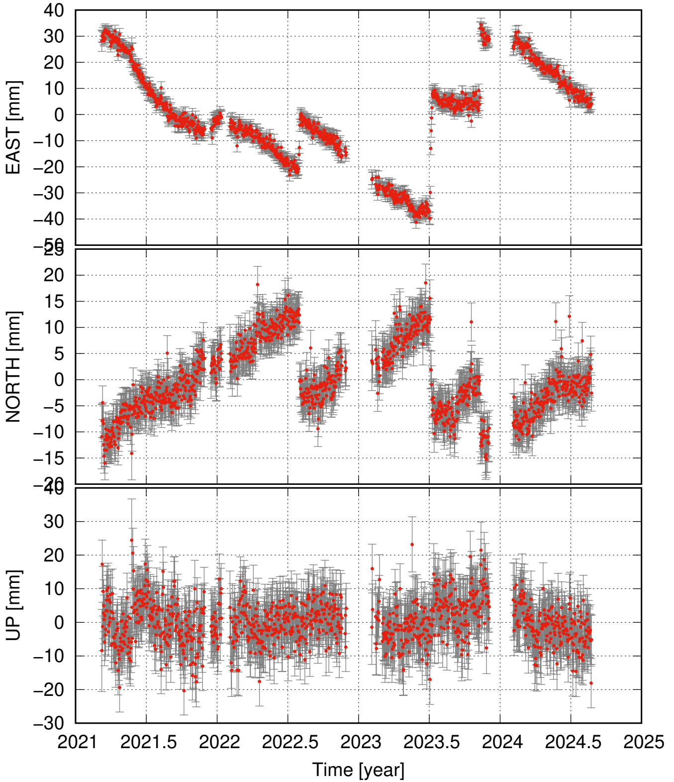
KLVC residual time series
