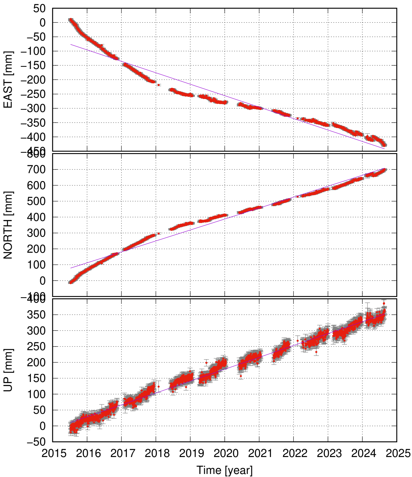
KISA (64.67, -17.56) time series (ITRF 2014) v_e = -40.04 \pm 3.19 ; v_n = 68.96 \pm 3.29 ; v_u = 37.39 \pm 1.24 mm/yr
