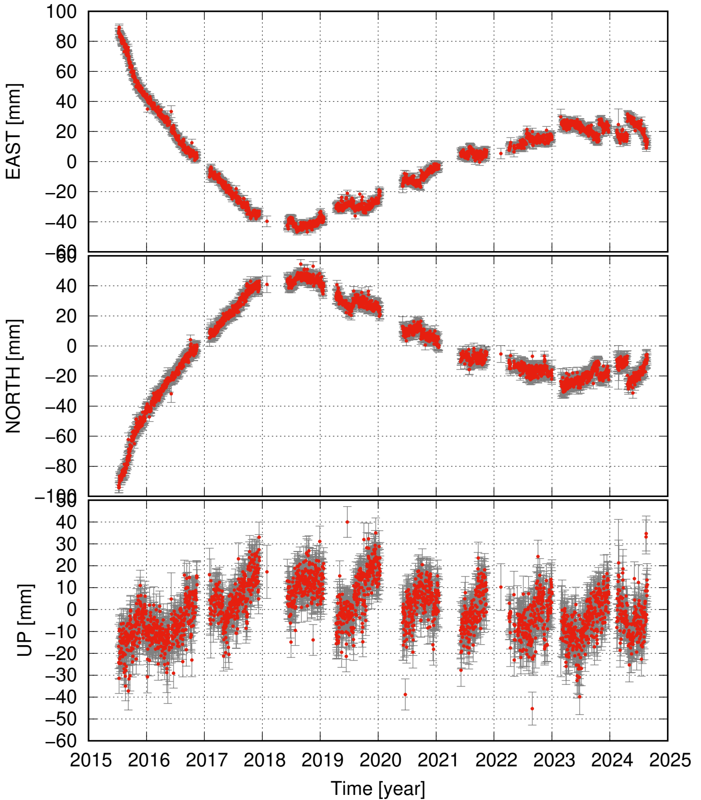
KISA residual time series (some major events removed as well)
