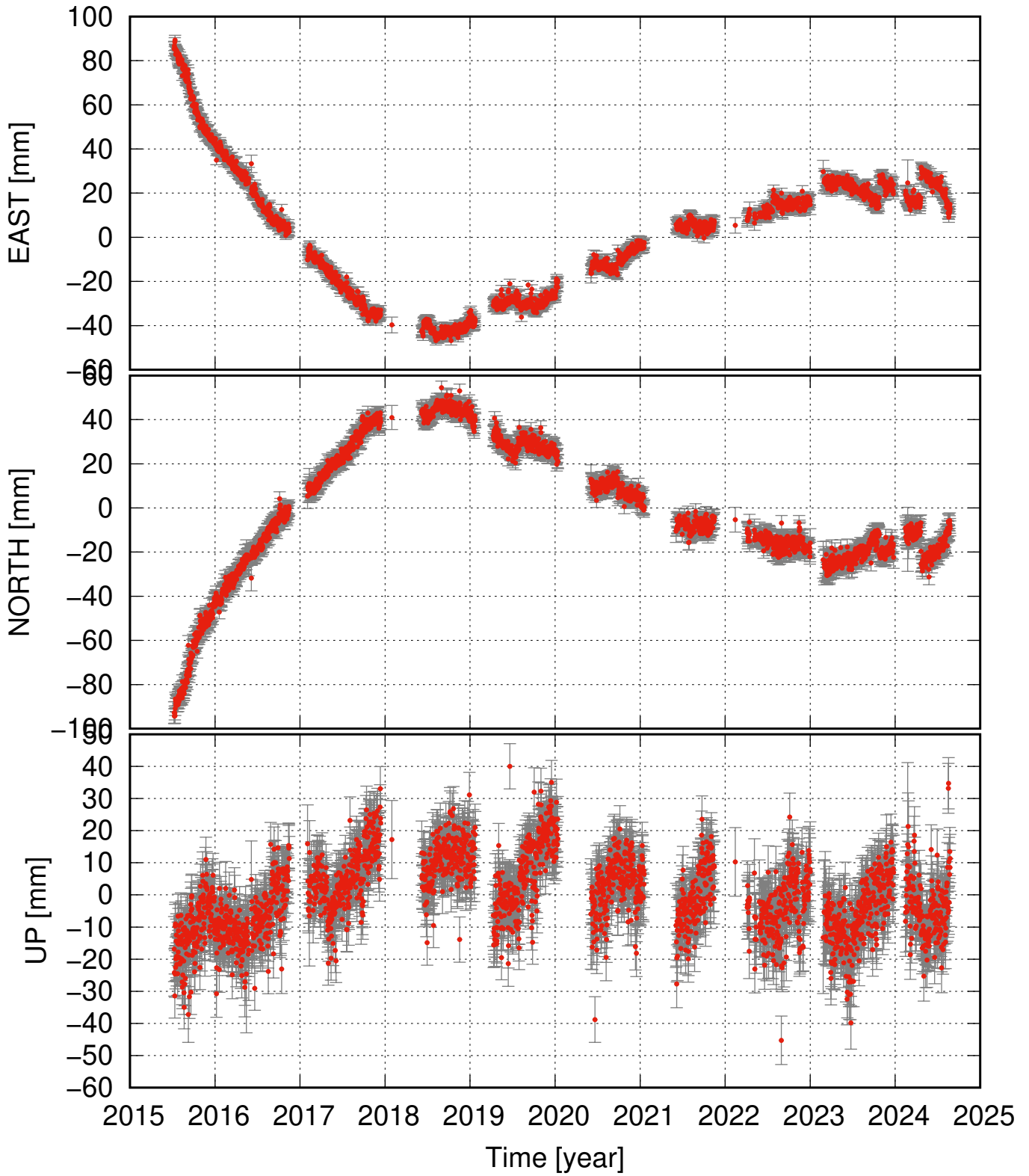
KISA residual time series
