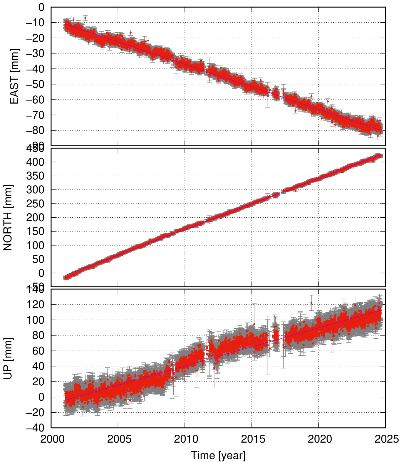
KIDJ (64.00, -20.77) time series (ITRF 2014) v_e = -2.92 \pm 0.08 ; v_n = 18.46 \pm 0.14 ; v_u = 4.96 \pm 0.30 mm/yr
