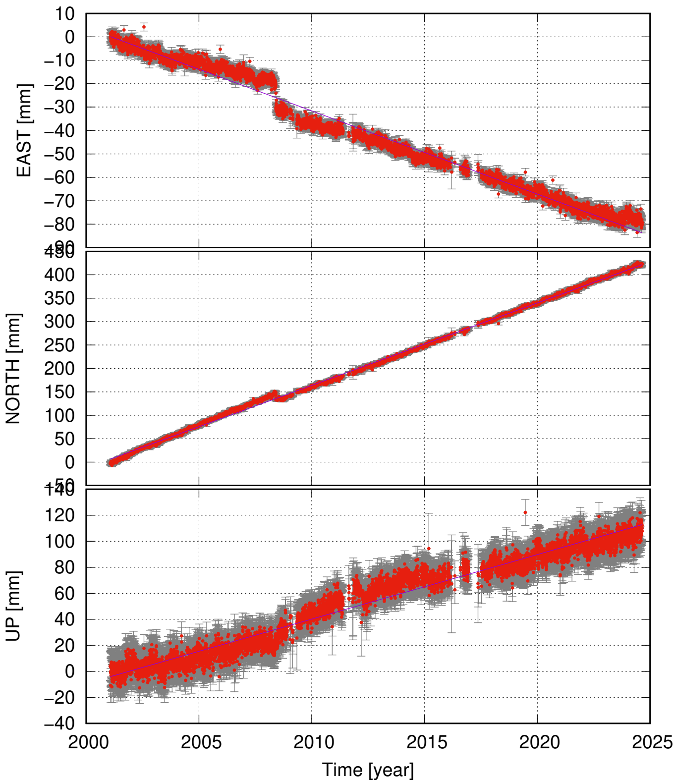
KIDJ (64.00, -20.77) time series (ITRF 2014) v_e = -3.56 \pm 0.14 ; v_n = 17.61 \pm 0.20 ; v_u = 4.96 \pm 0.30 mm/yr
