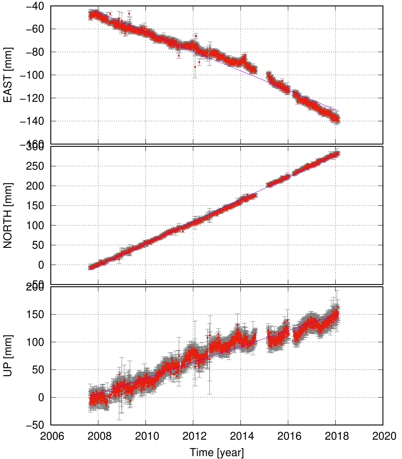
KIDC (65.02, -17.94) time series (ITRF 2014) v_e = -8.47 \pm 0.41 ; v_n = 28.05 \pm 0.36 ; v_u = 14.24 \pm 0.96 mm/yr
