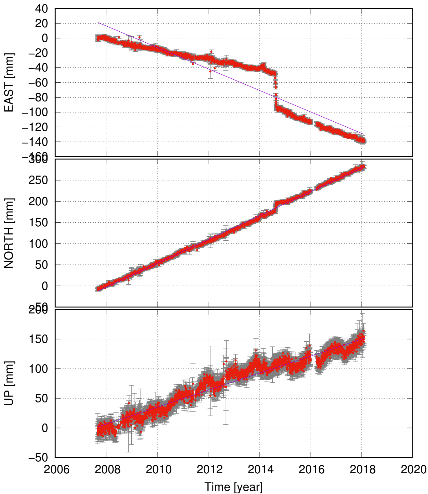
KIDC (65.02, -17.94) time series (ITRF 2014) v_e = -14.48 \pm 1.52 ; v_n = 28.13 \pm 0.39 ; v_u = 14.31 \pm 0.94 mm/yr
