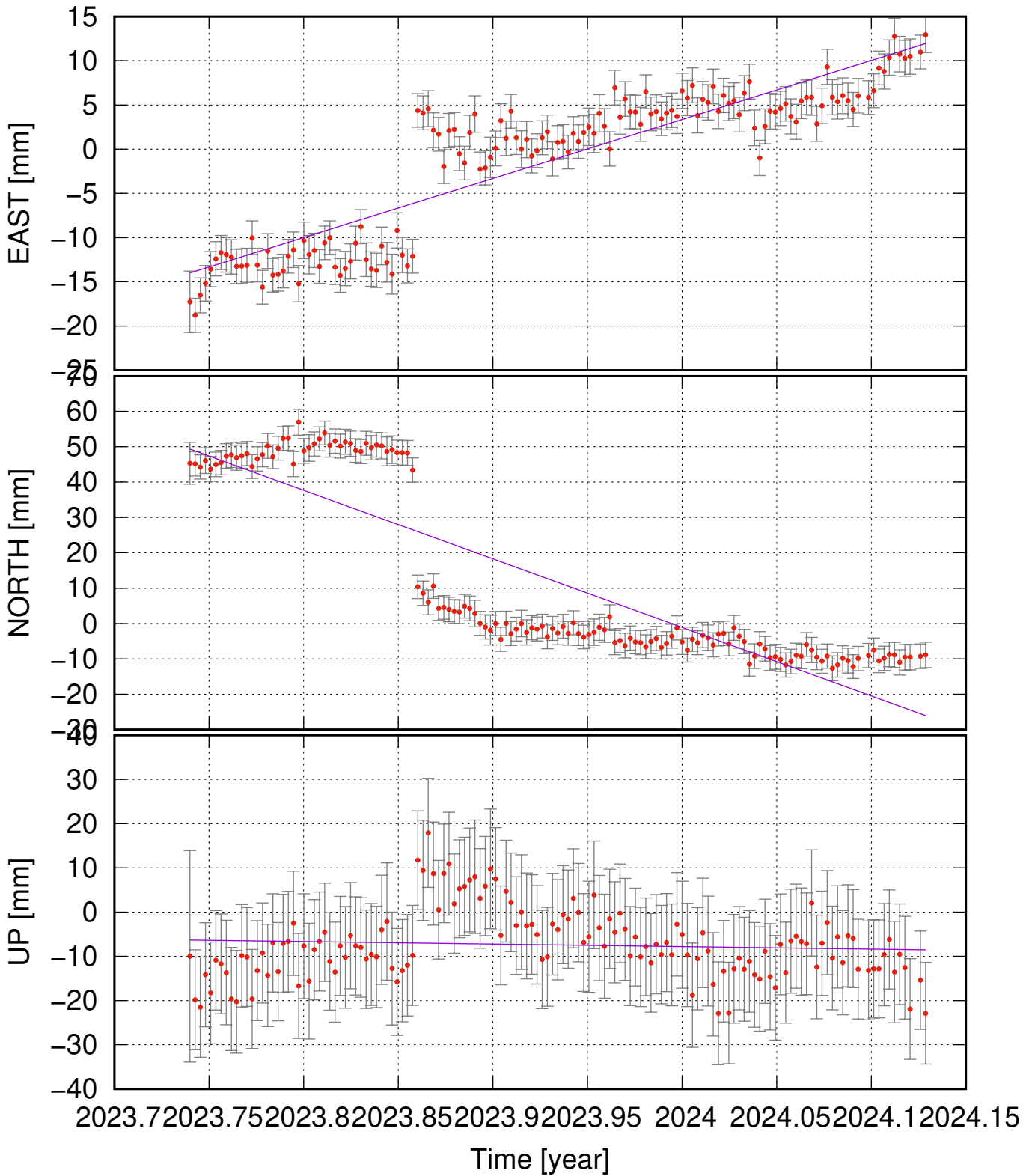
KEIC (63.93, -22.19) time series (ITRF 2014) v_e = 66.73 \pm 9.48 ; v_n = -193.94 \pm 31.92 ; v_u = -5.79 \pm 20.11 mm/yr
