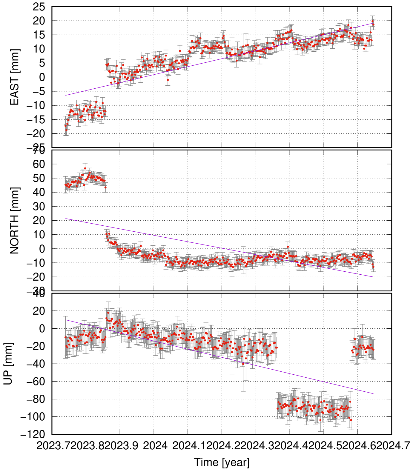
KEIC (63.93, -22.19) time series (ITRF 2014) v_e = 28.29 \pm 4.92 ; v_n = -45.79 \pm 16.36 ; v_u = -92.42 \pm 26.93 mm/yr
