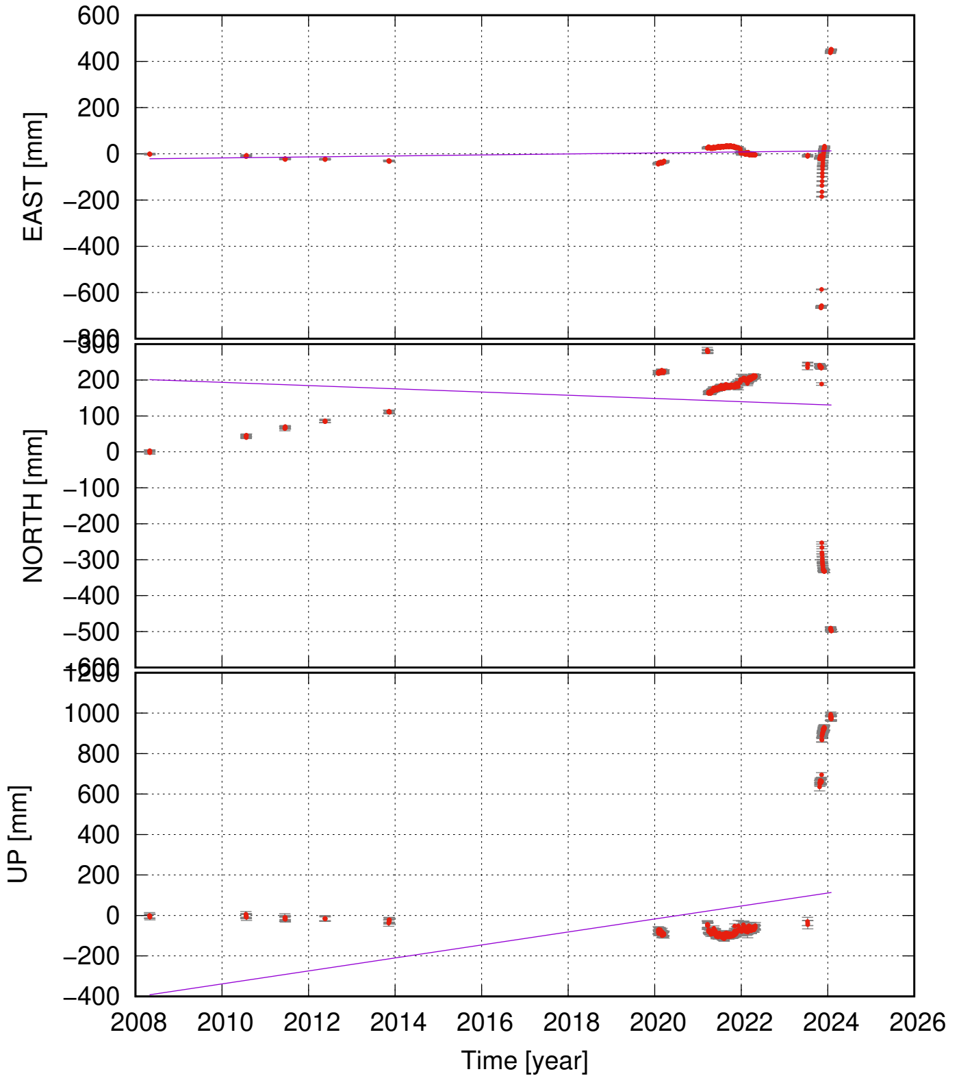
KAST (63.88, -22.32) time series (ITRF 2014) v_e = 2.18 \pm 6.86 ; v_n = -4.49 \pm 9.68 ; v_u = 32.12 \pm 17.96 mm/yr
