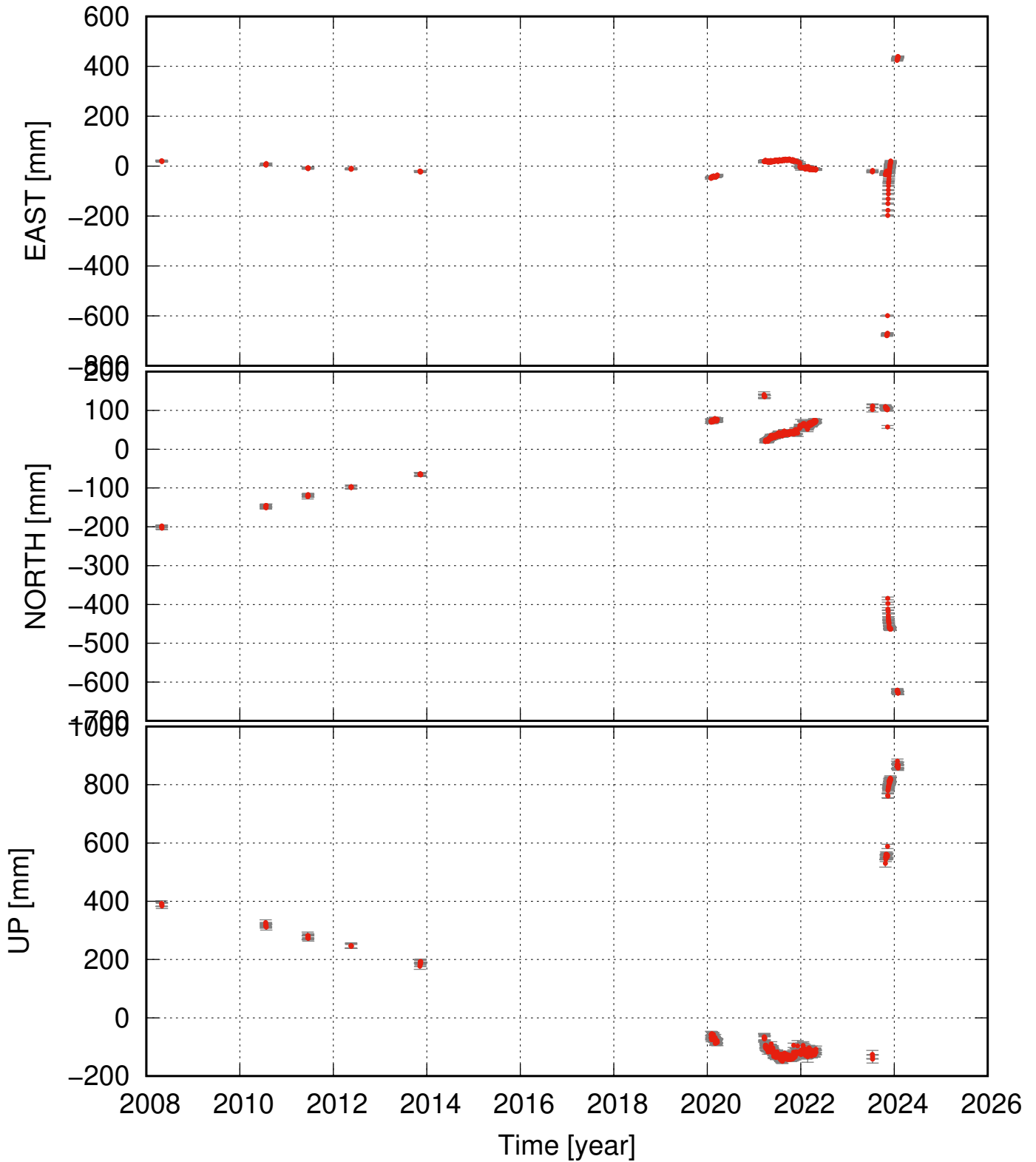
KAST residual time series (some major events removed as well)
