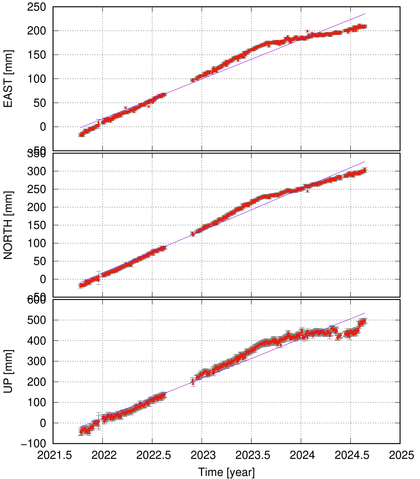
KASC (65.06, -16.76) time series (ITRF 2014) v_e = 82.73 \pm 4.42 ; v_n = 116.99 \pm 4.26 ; v_u = 193.07 \pm 10.83 mm/yr
