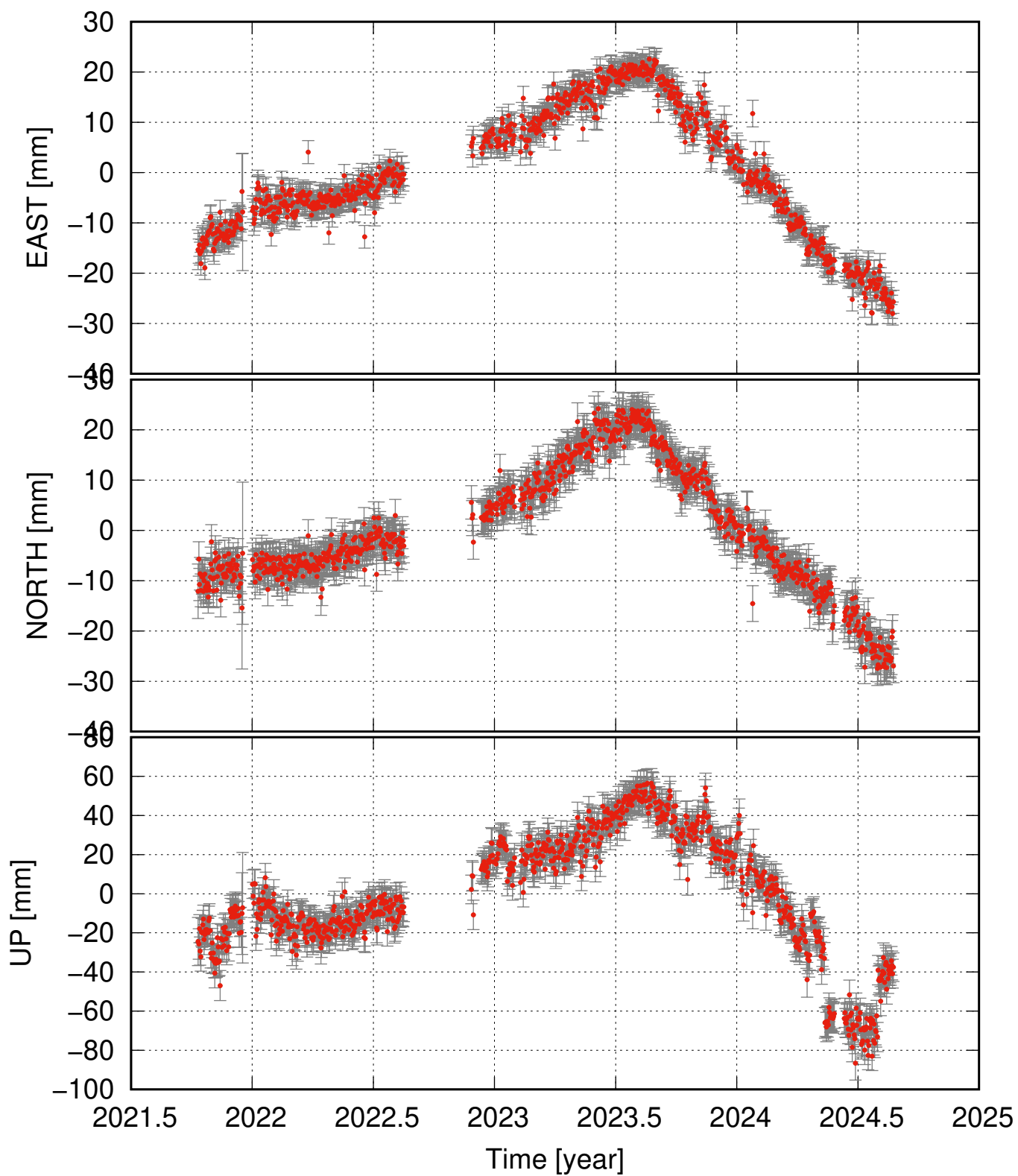
KASC residual time series
