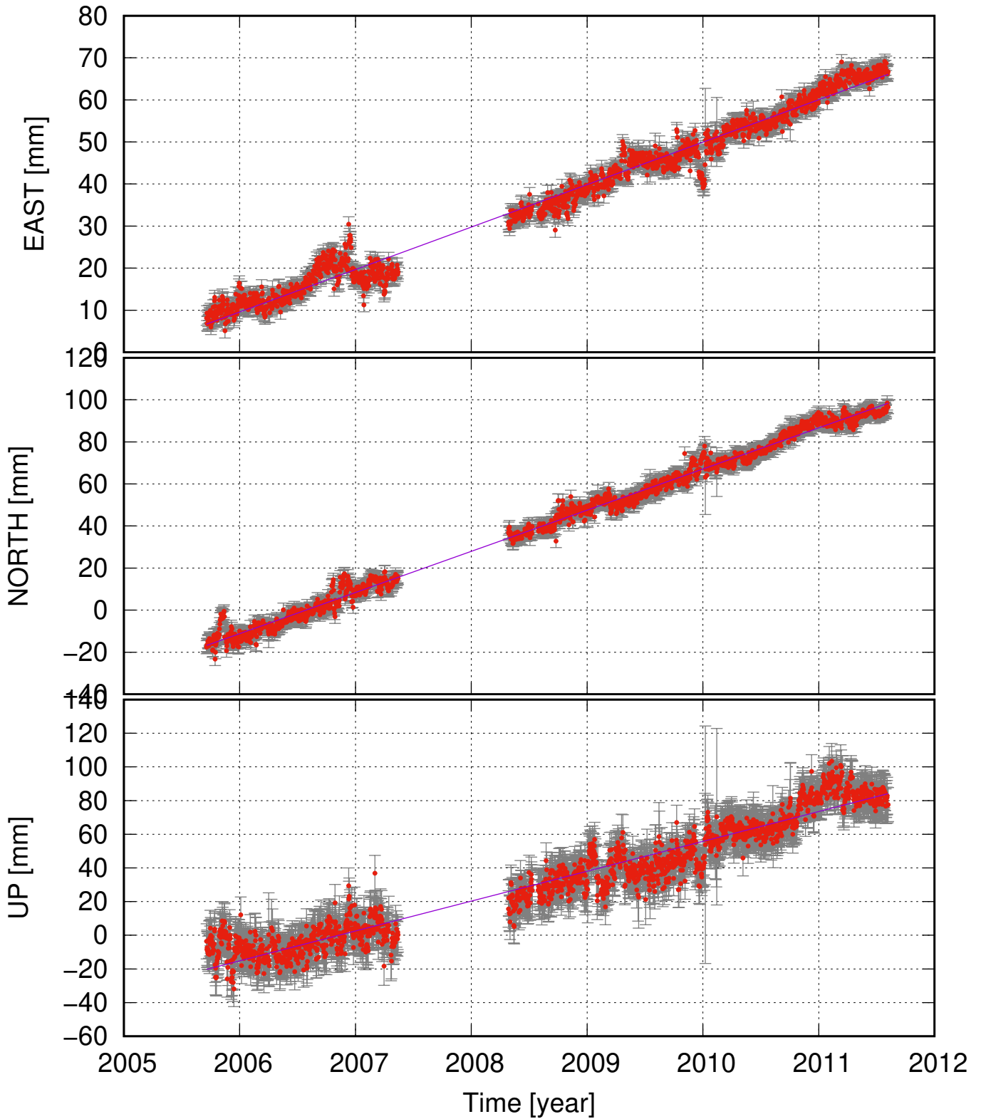
KARV (64.93, -15.84) time series (ITRF 2014) v_e = 10.09 \pm 0.43 ; v_n = 19.56 \pm 0.49 ; v_u = 17.74 \pm 1.47 mm/yr
