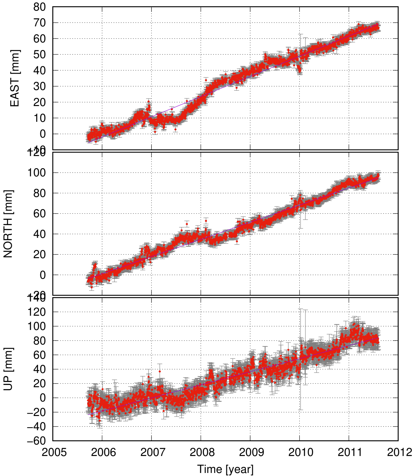
KARV (64.93, -15.84) time series (ITRF 2014) v_e = 12.70 \pm 0.61 ; v_n = 16.76 \pm 0.71 ; v_u = 18.30 \pm 1.59 mm/yr
