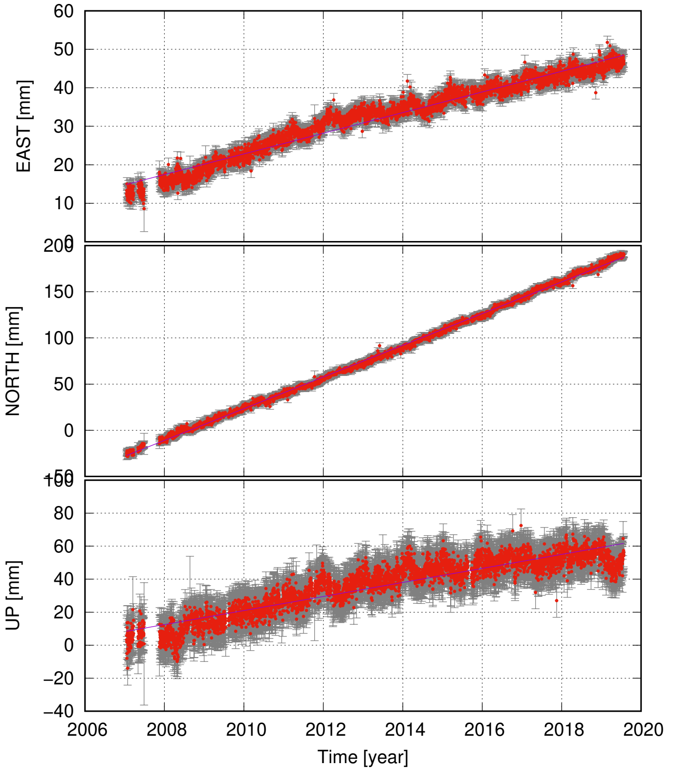
KALT (63.90, -20.66) time series (ITRF 2014) v_e = 2.68 \pm 0.15 ; v_n = 17.15 \pm 0.20 ; v_u = 4.26 \pm 0.52 mm/yr
