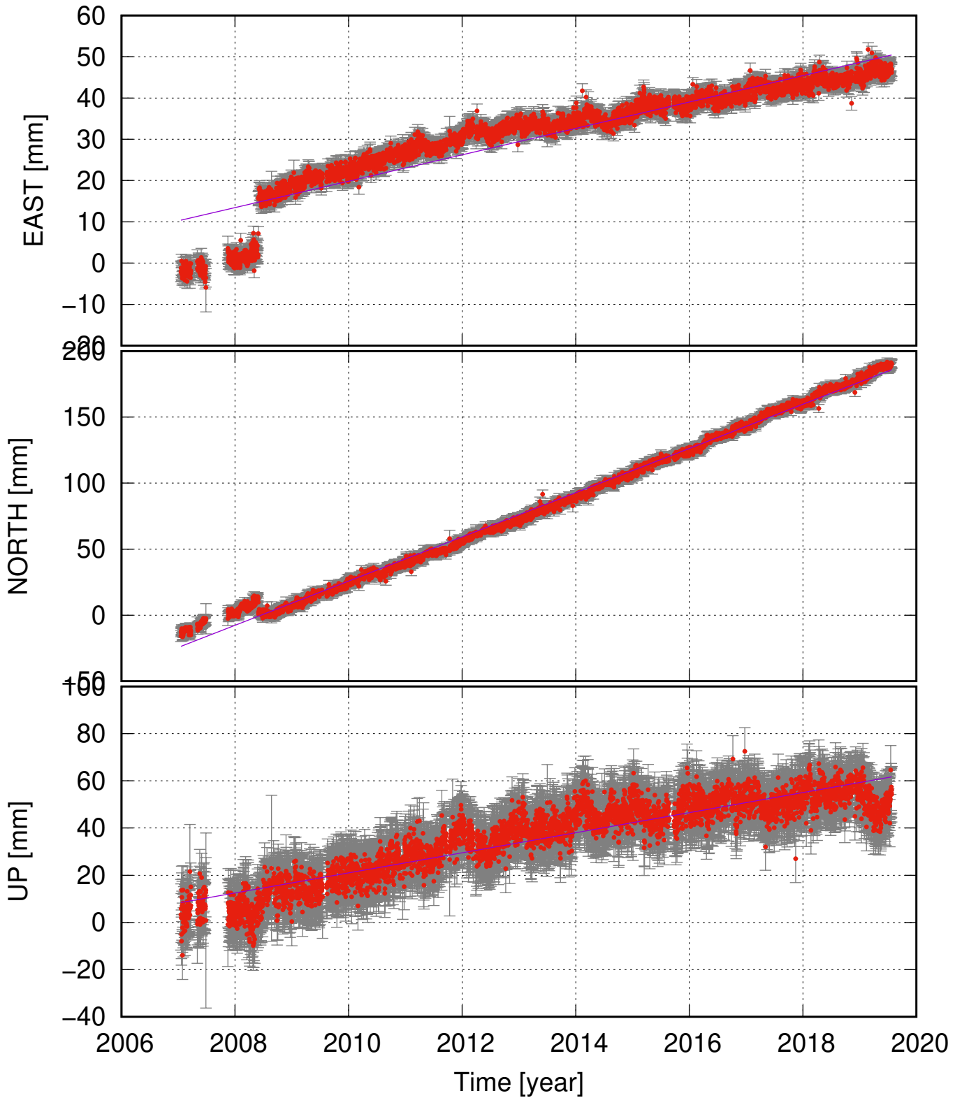
KALT (63.90, -20.66) time series (ITRF 2014) v_e = 3.19 \pm 0.35 ; v_n = 16.73 \pm 0.34 ; v_u = 4.26 \pm 0.52 mm/yr
