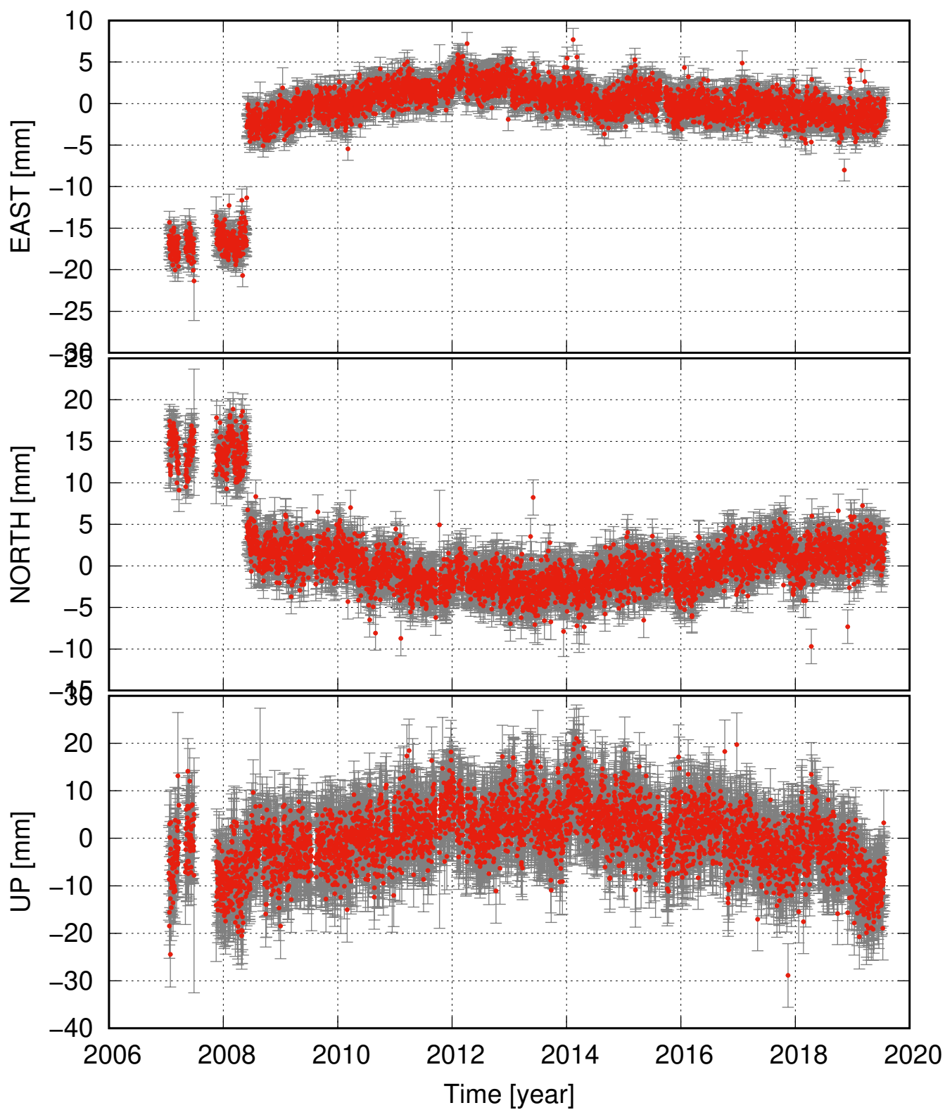
KALT detrended and seasonal signal removed
