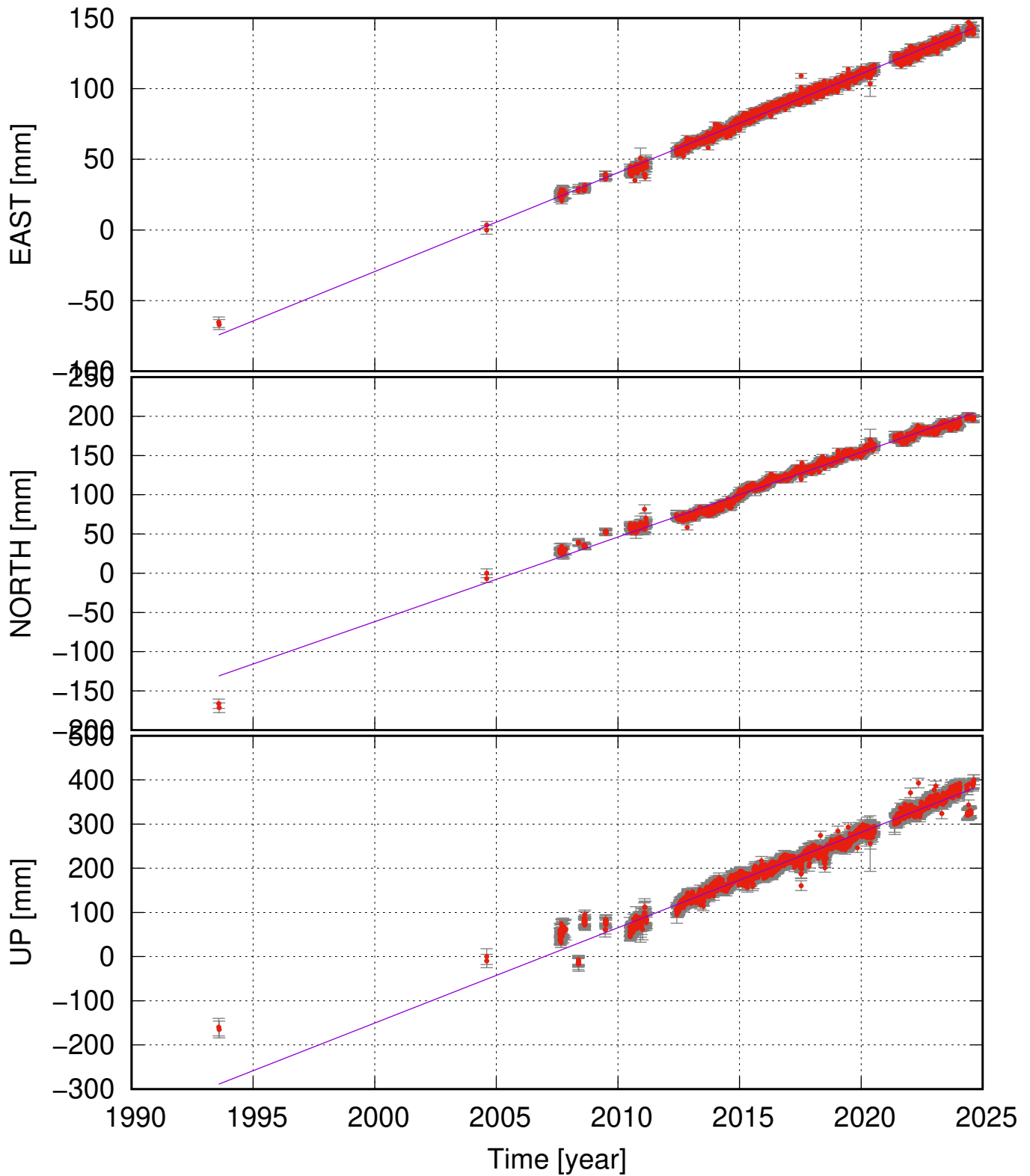
KALF (63.95, -17.69) time series (ITRF 2014) v_e = 7.00 \pm 0.06 ; v_n = 10.78 \pm 0.15 ; v_u = 21.57 \pm 0.36 mm/yr
