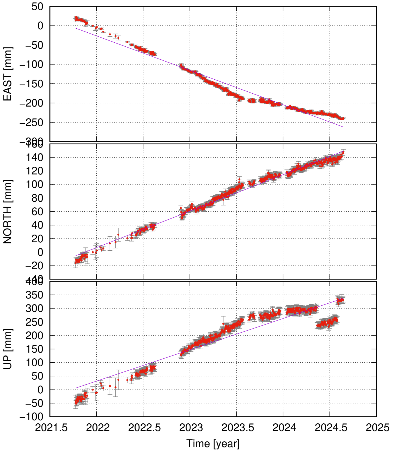
JONC (65.05, -16.83) time series (ITRF 2014) v_e = -89.11 \pm 4.84 ; v_n = 53.86 \pm 1.65 ; v_u = 115.59 \pm 11.83 mm/yr
