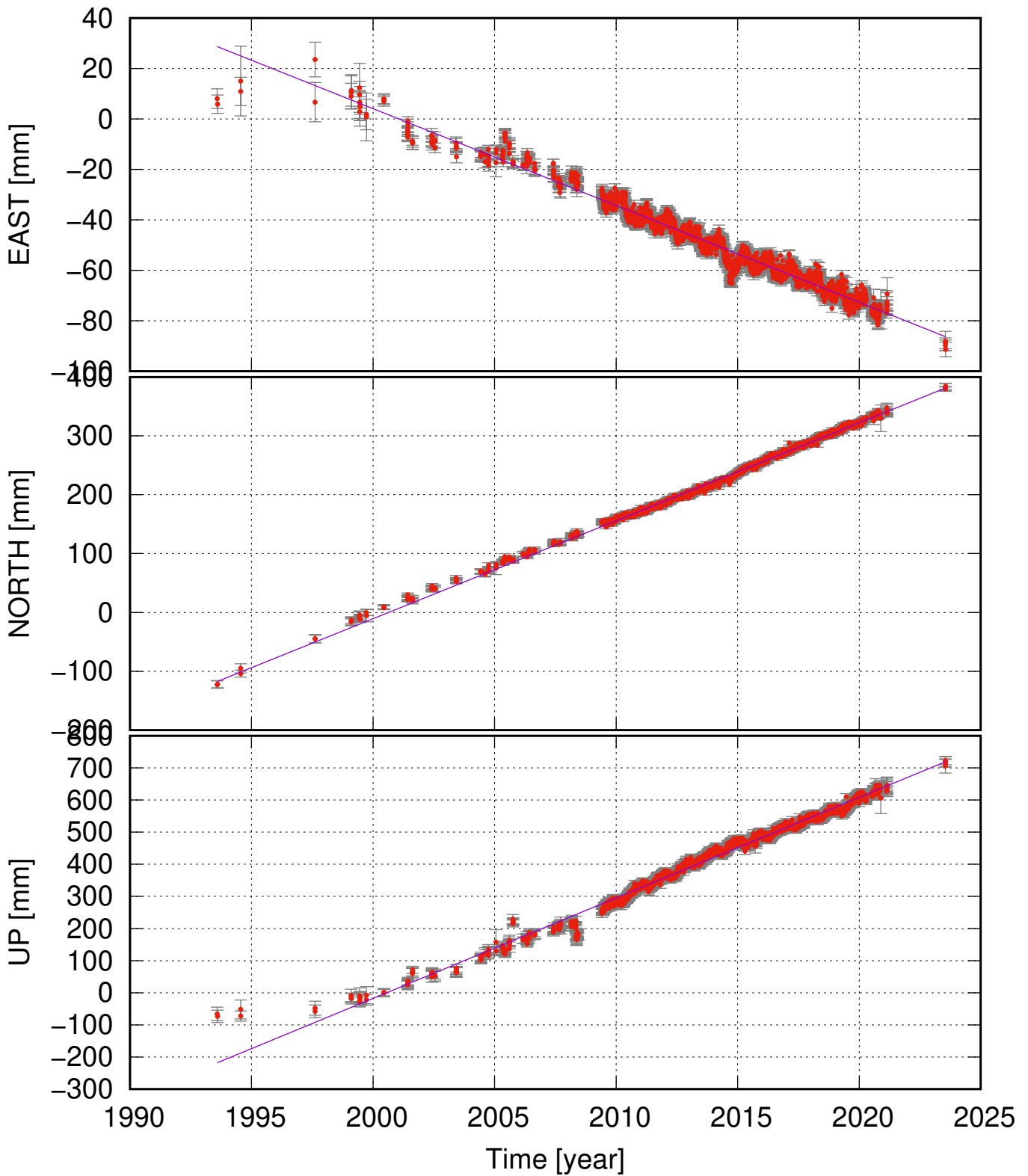
JOKU (64.31, -18.24) time series (ITRF 2014) v_e = -3.84 \pm 0.09 ; v_n = 16.65 \pm 0.12 ; v_u = 31.28 \pm 0.45 mm/yr
