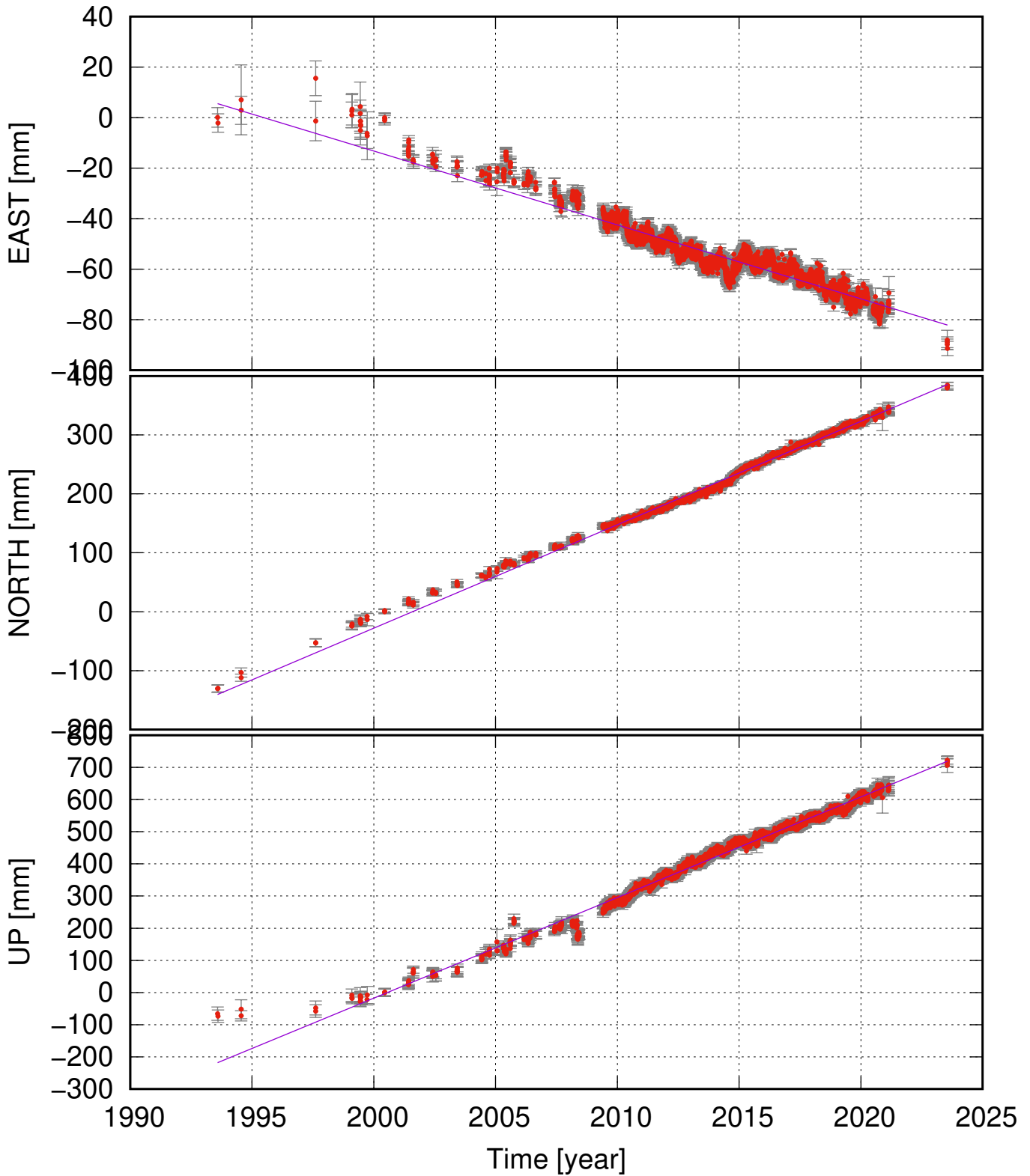
JOKU (64.31, -18.24) time series (ITRF 2014) v_e = -2.93 \pm 0.11 ; v_n = 17.55 \pm 0.17 ; v_u = 31.28 \pm 0.45 mm/yr
