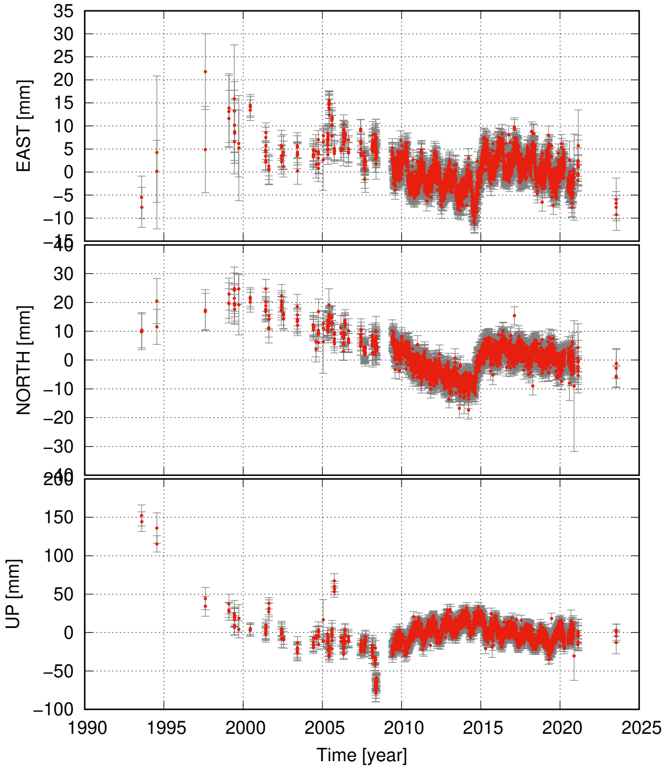
JOKU residual time series
