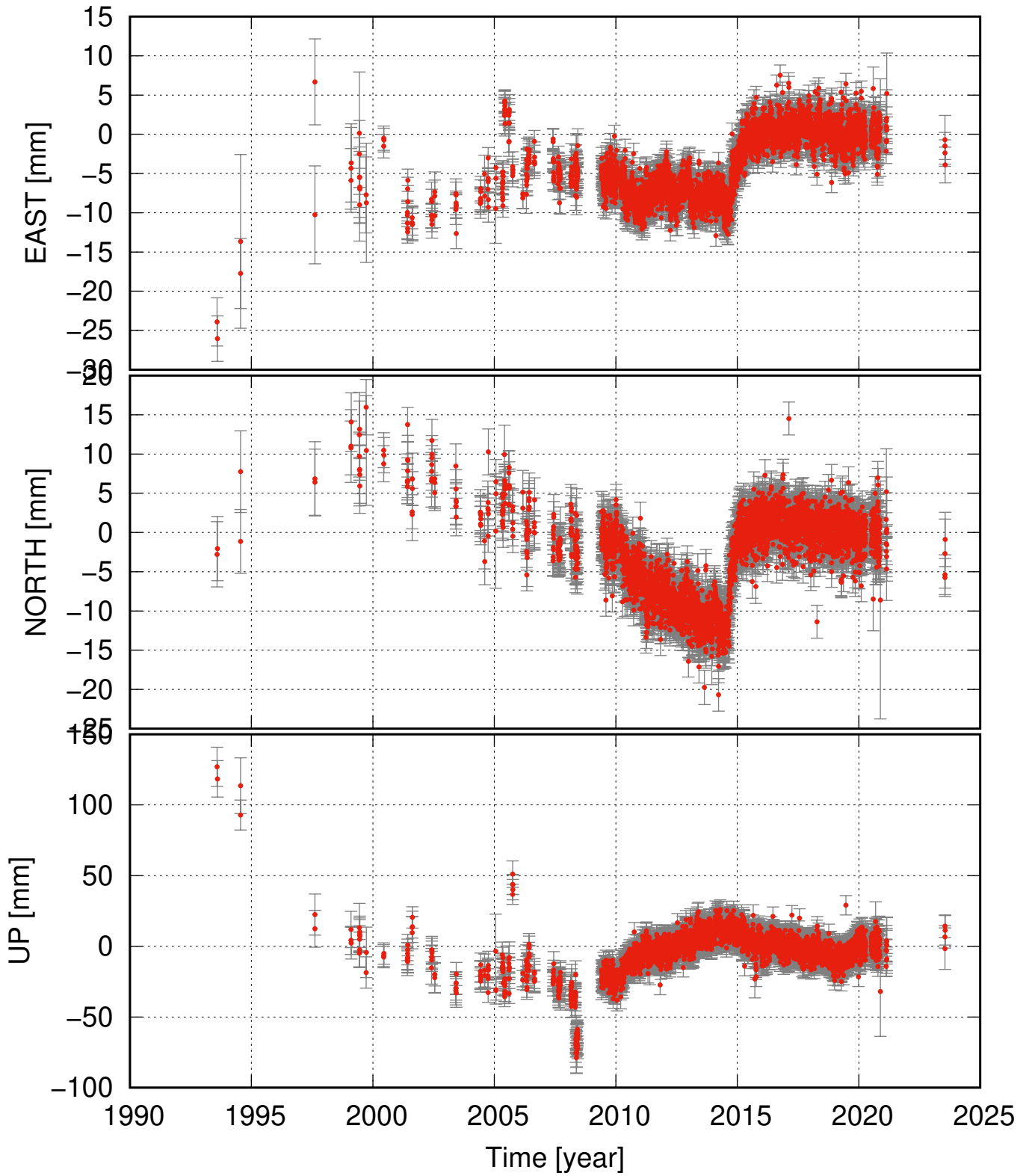
JOKU detrended and seasonal signal removed
