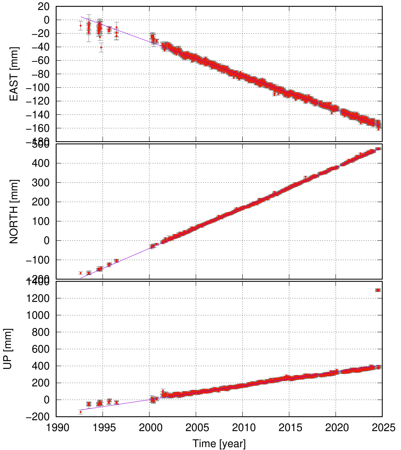
ISAK (64.12, -19.75) time series (ITRF 2014) v_e = -5.02 \pm 0.06 ; v_n = 20.87 \pm 0.09 ; v_u = 16.46 \pm 1.94 mm/yr
