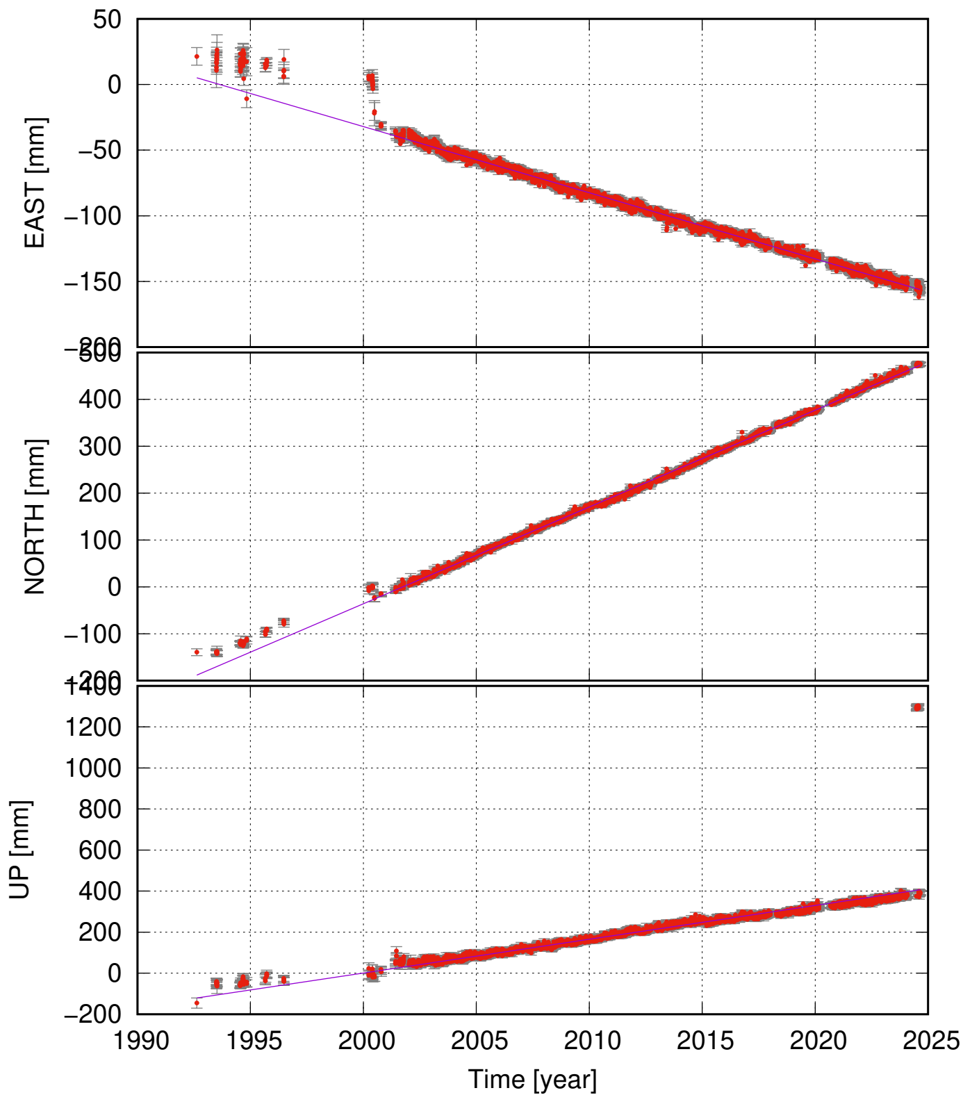
ISAK (64.12, -19.75) time series (ITRF 2014) v_e = -5.04 \pm 0.10 ; v_n = 20.64 \pm 0.13 ; v_u = 16.46 \pm 1.94 mm/yr
