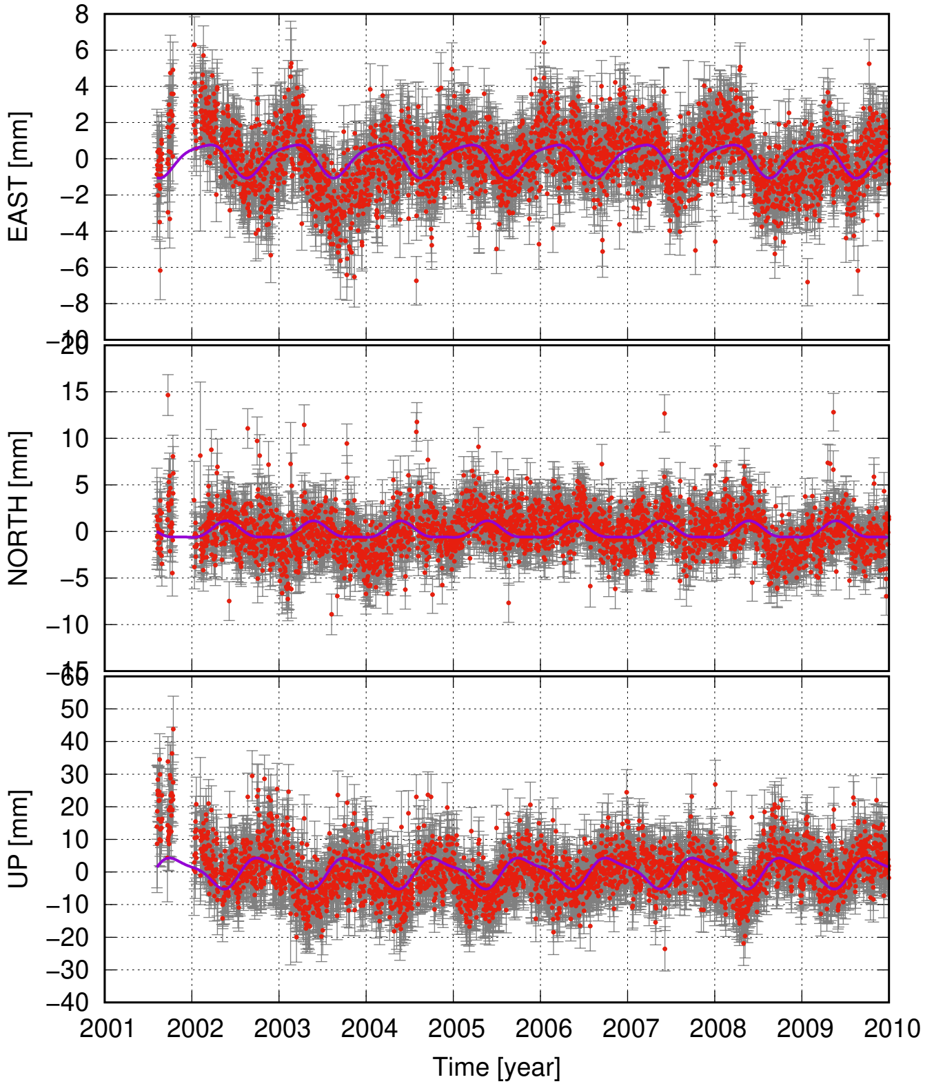
ISAK seasonal fit
