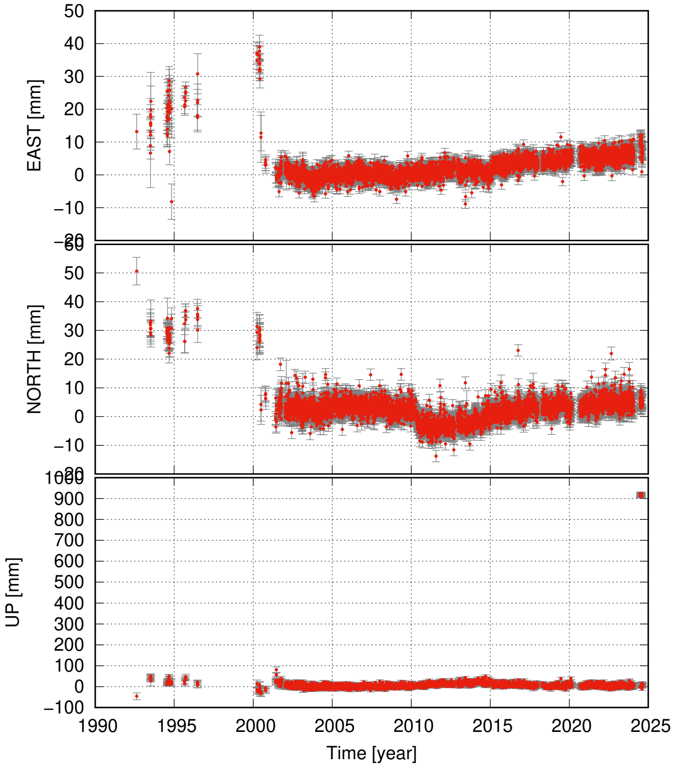
ISAK detrended and seasonal signal removed
