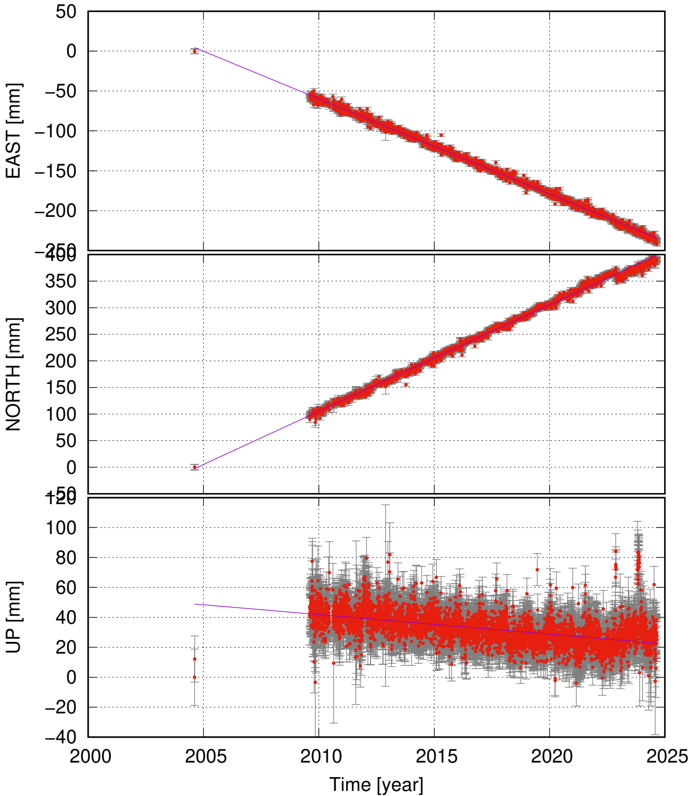
ISAF (66.07, -23.12) time series (ITRF 2014) v_e = -11.92 \pm 0.12 ; v_n = 20.01 \pm 0.22 ; v_u = -1.31 \pm 0.45 mm/yr
