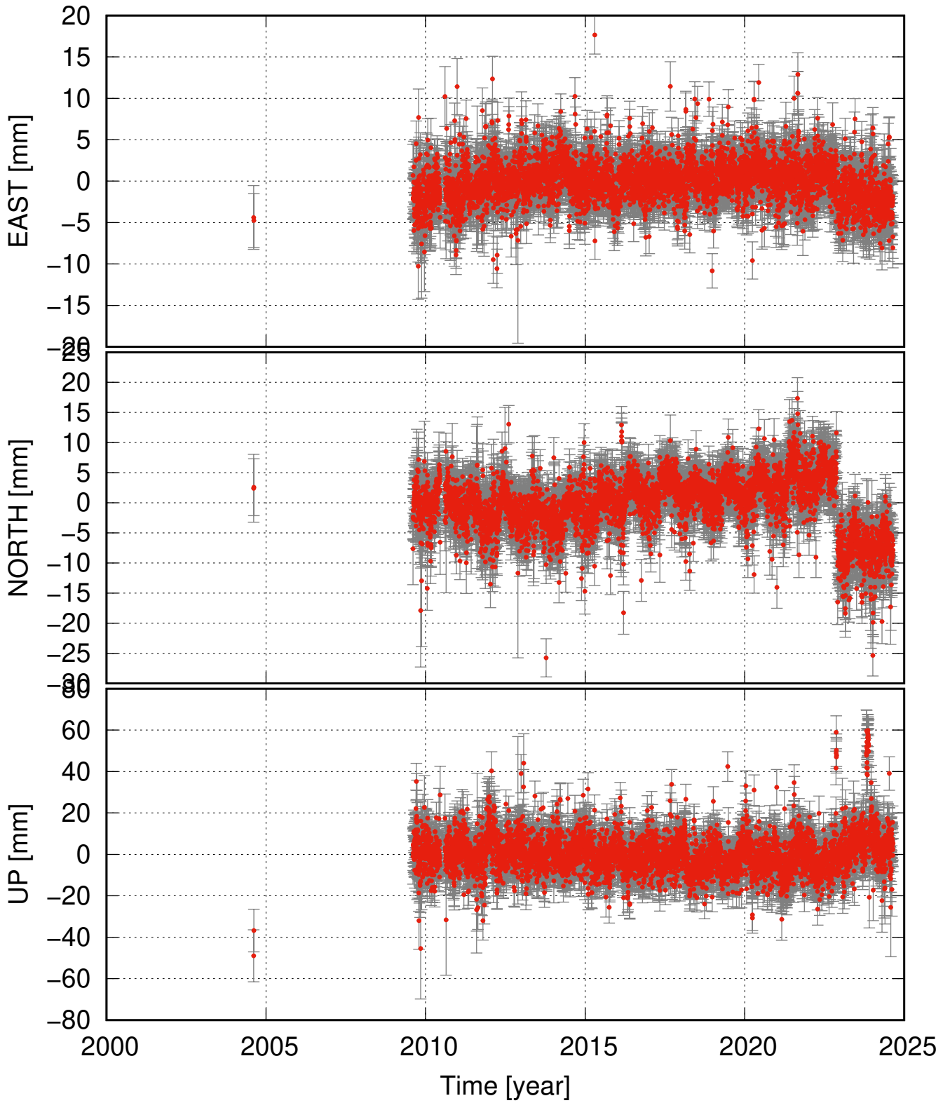
ISAF residual time series (some major events removed as well)
