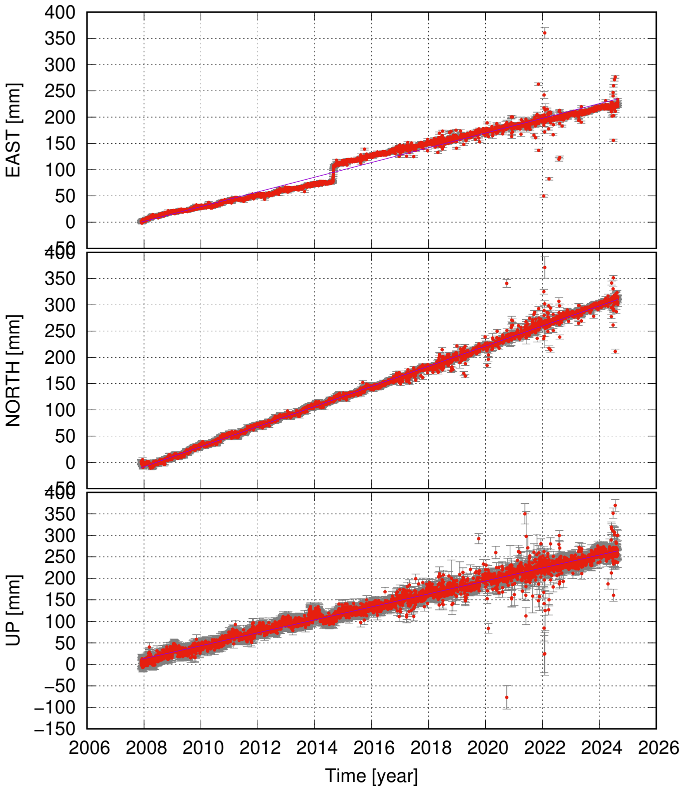
INTA (64.94, -15.78) time series (ITRF 2014) v_e = 14.01 \pm 0.58 ; v_n = 19.14 \pm 0.30 ; v_u = 15.08 \pm 0.70 mm/yr
