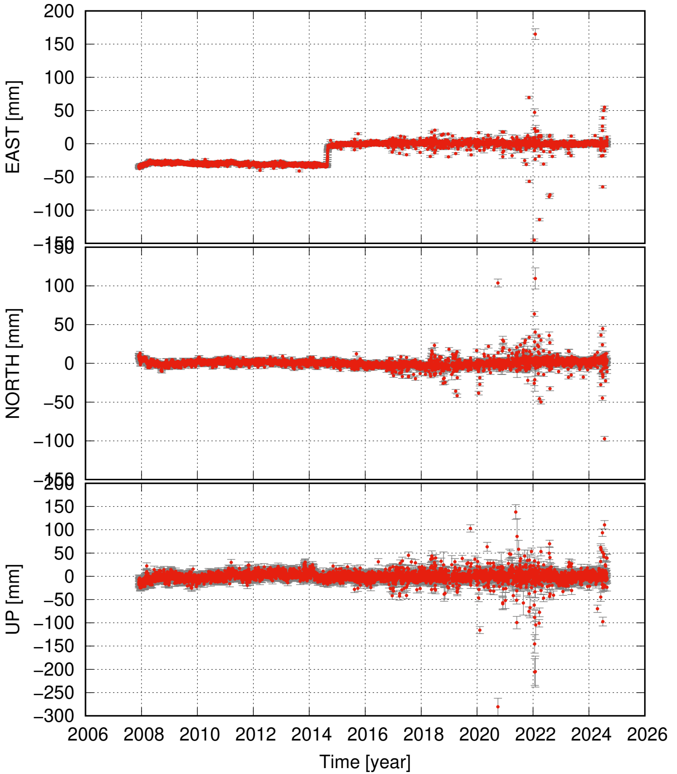
INTA detrended and seasonal signal removed
