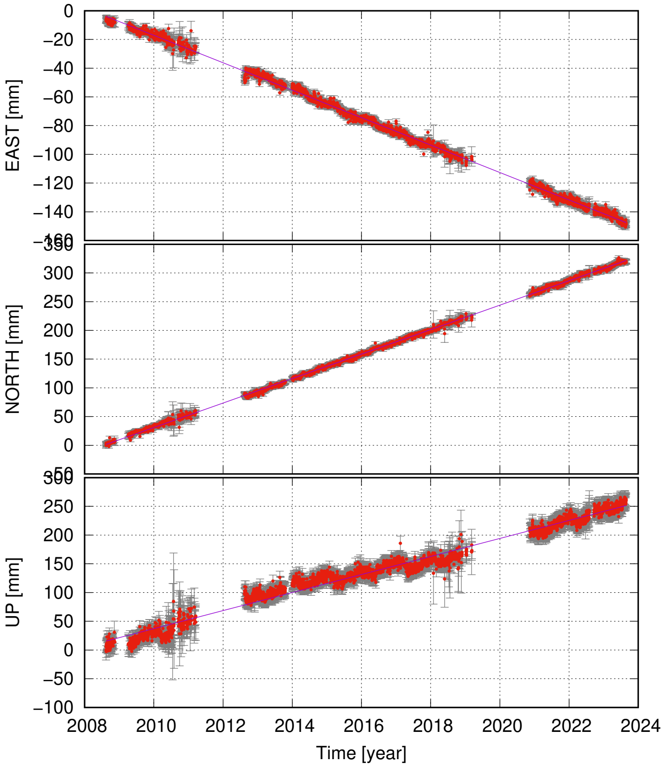
INSK (64.68, -19.53) time series (ITRF 2014) v_e = -9.55 \pm 0.12 ; v_n = 21.31 \pm 0.15 ; v_u = 15.70 \pm 0.67 mm/yr
