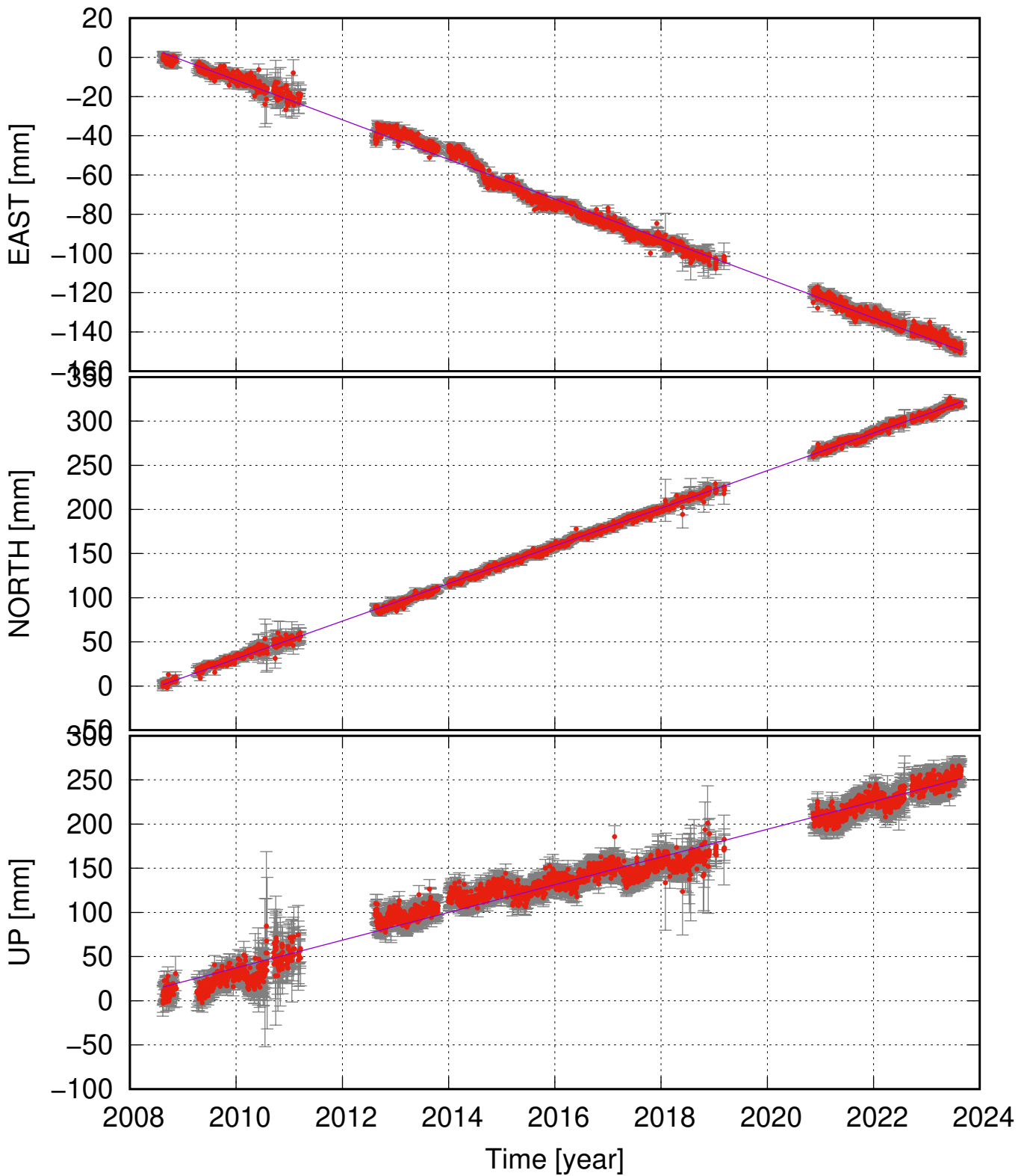
INSK (64.68, -19.53) time series (ITRF 2014) ve = -10.10 \pm 0.19 ; vn = 21.31 \pm 0.15 ; vu = 15.70 \pm 0.67 mm/yr
