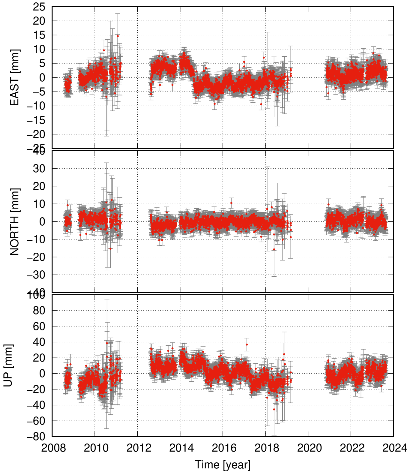
INSK residual time series
