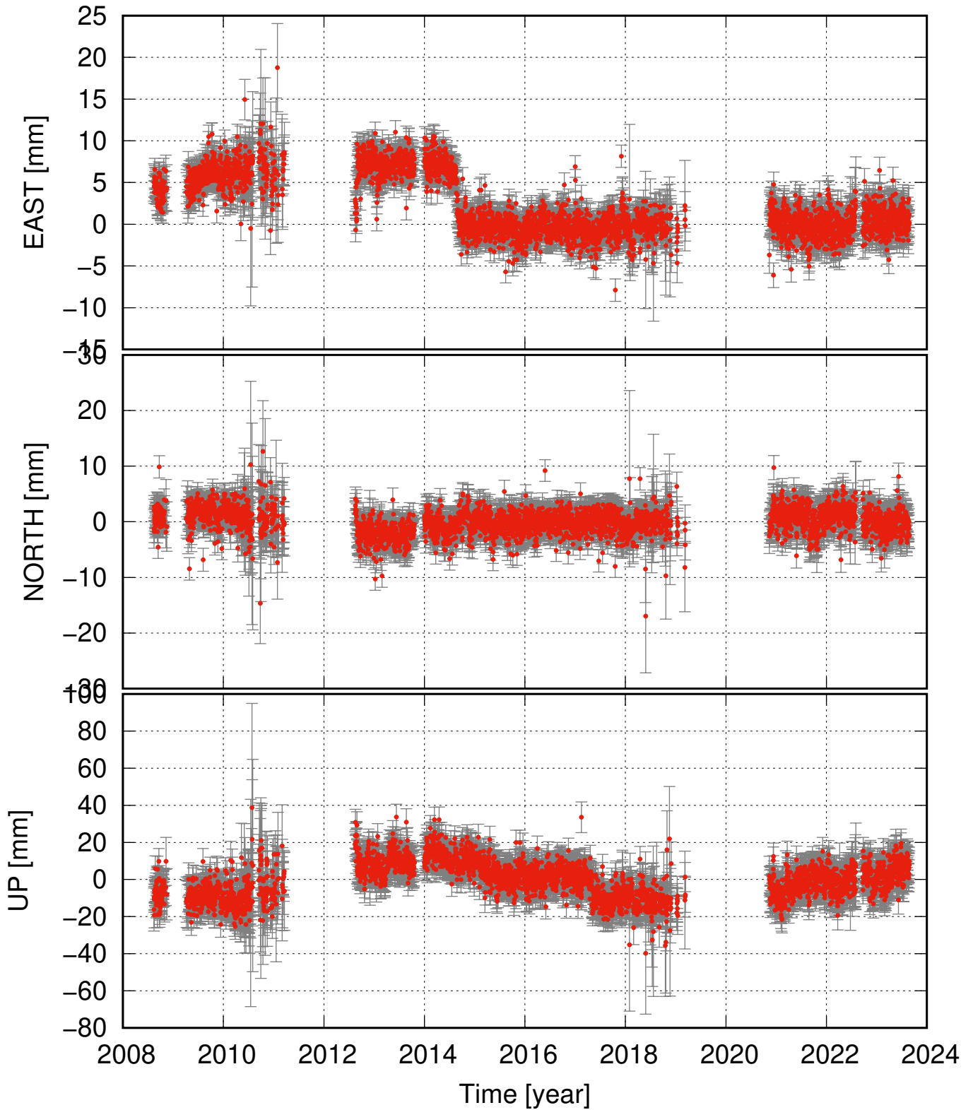
INSK detrended and seasonal signal removed
