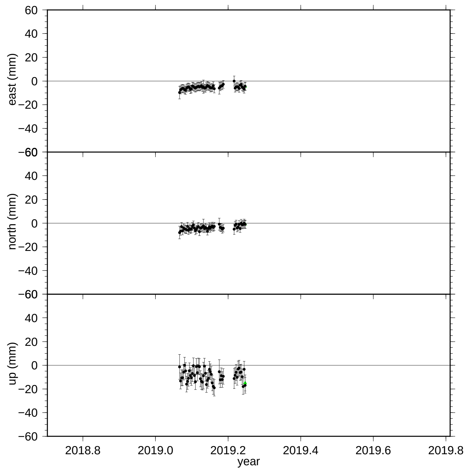
INGC time series (ITRF 2008), last 400 days
