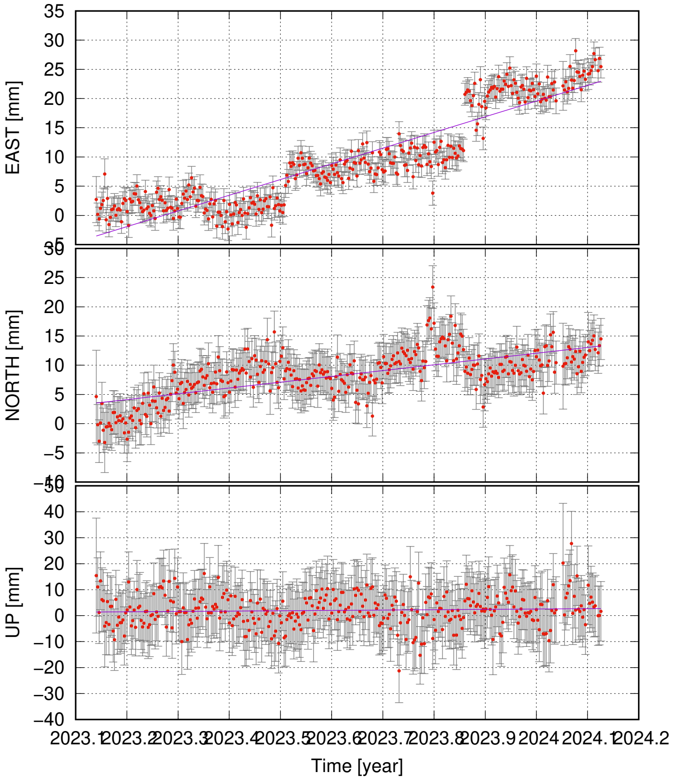
HVSK (63.94, -21.71) time series (ITRF 2014) v_e = 26.87 \pm 3.37 ; v_n = 9.92 \pm 3.01 ; v_u = 1.33 \pm 6.17 mm/yr
