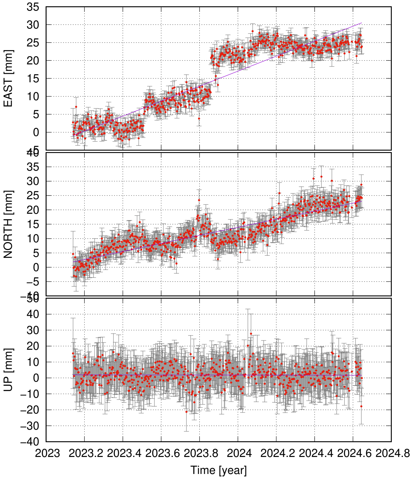
HVSK (63.94, -21.71) time series (ITRF 2014) v_e = 20.89 \pm 2.42 ; v_n = 14.05 \pm 2.07 ; v_u = -0.15 \pm 3.90 mm/yr
