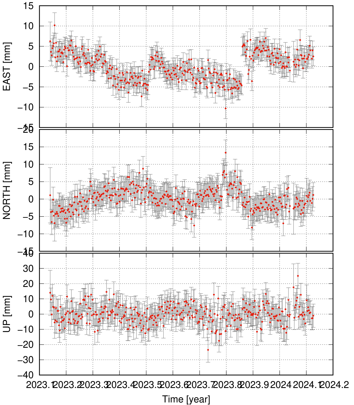
HVSK residual time series (some major events removed as well)
