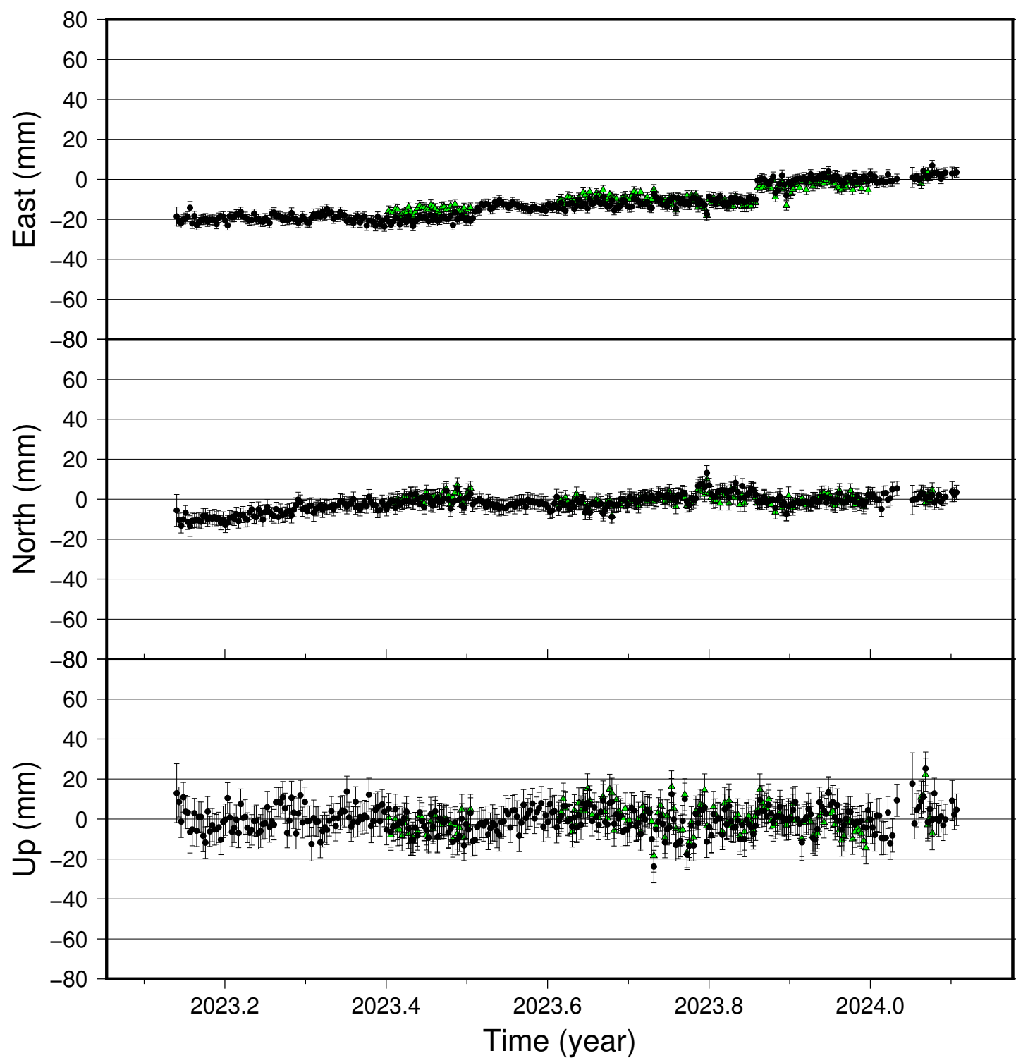
HVSK time series (IGS 2014), last 400 days
