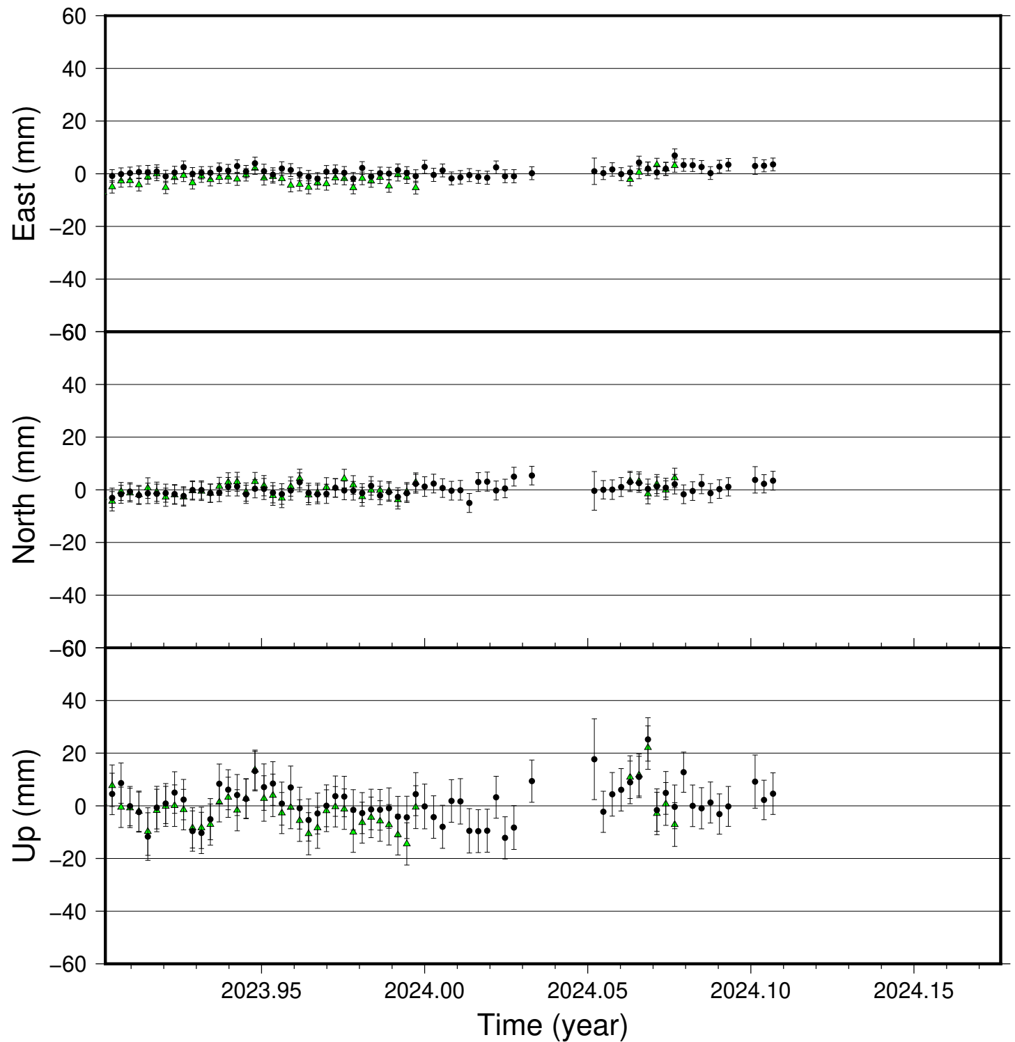
HVSK time series (IGS 2014), last 100 days
