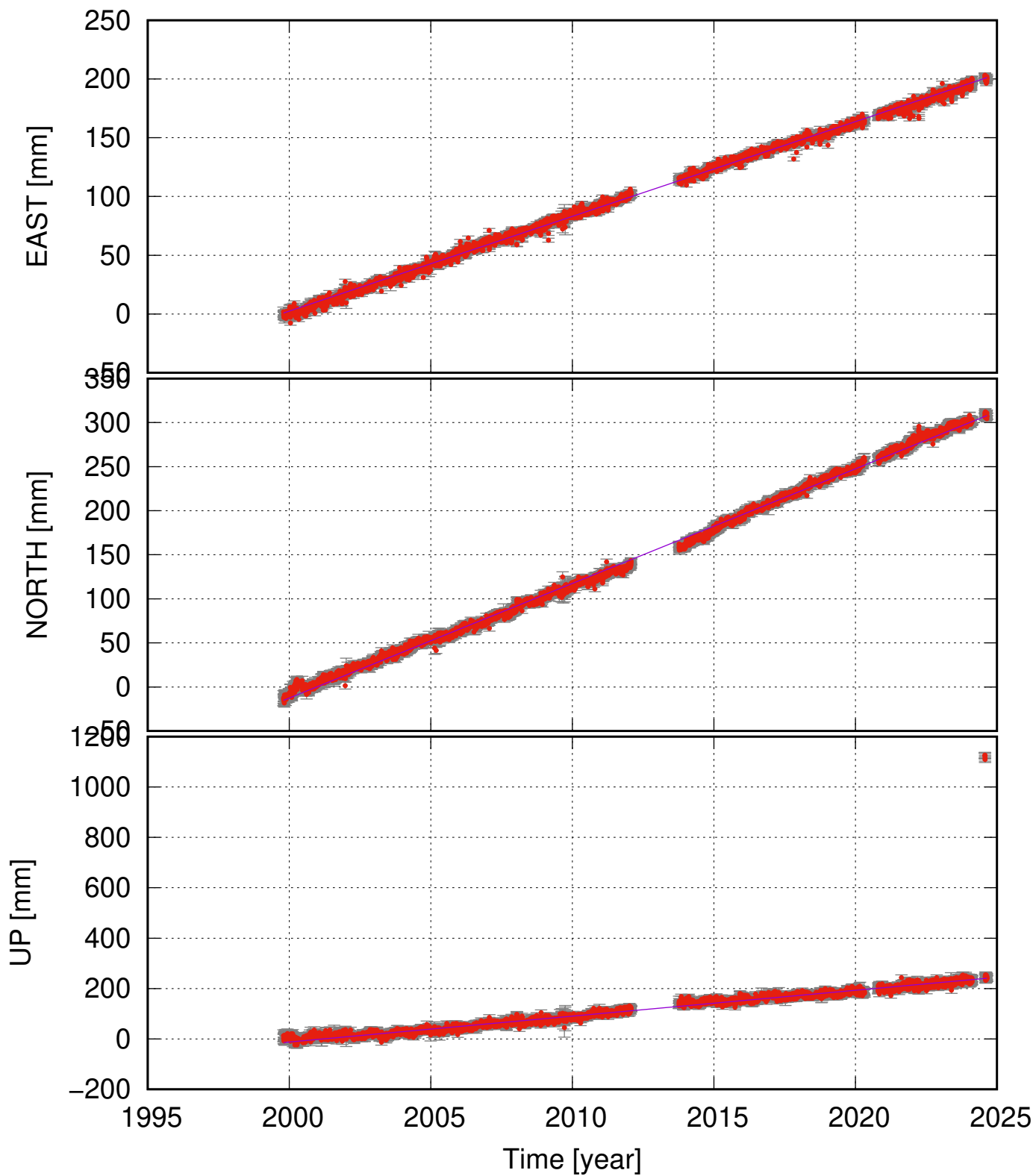
HVOL (63.53, -18.85) time series (ITRF 2014) ve = 8.06 +- 0.09; vn = 13.01 +- 0.17; vu = 10.28 +- 0.98 mm/yr
