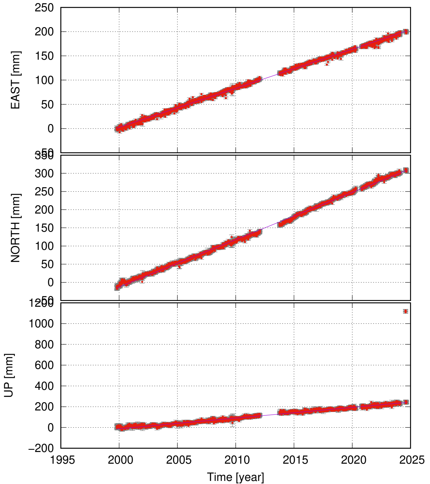
HVOL (63.53, -18.85) time series (ITRF 2014) ve = 8.06 \pm 0.09 ; vn = 13.01 \pm 0.17 ; vu = 10.28 \pm 0.98 mm/yr
