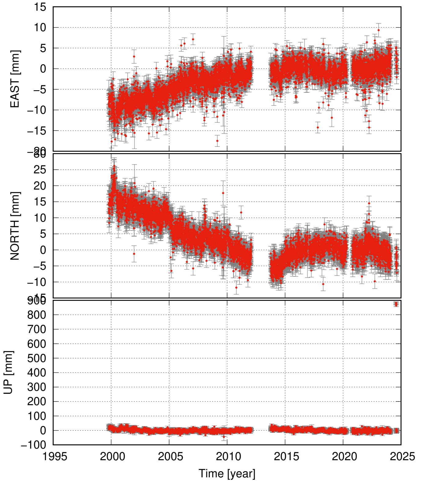
HVOL detrended and seasonal signal removed
